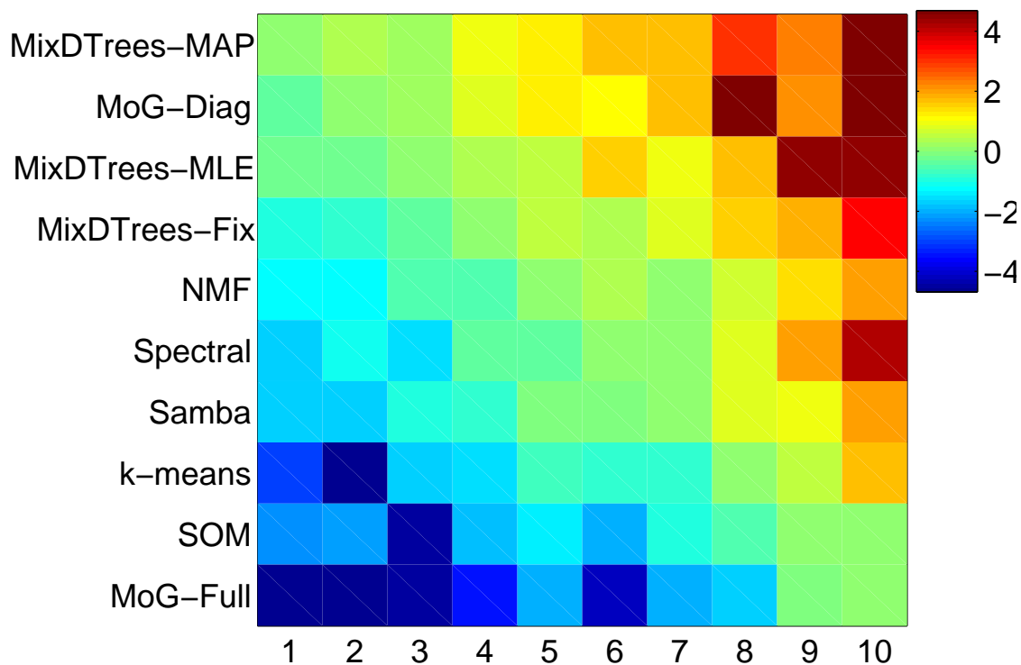
Figure 1: Heat-map plot displaying the comparison of GO enrichment for 10 distinct clustering methods. More precisely, entries in the plot correspond to \log(\#\{p\text{-value } m_y < p\text{-value } m_x\} / \#\{p\text{-value } m_y > p\text{-value } m_x\}) , where red (or blue) values indicate that the method on the y -axis ( m_y ) had a higher (or lower) count of enriched GO term than the method on the x -axis ( m_x ); numbers on the x -axis correspond to the methods in the y -axis.
