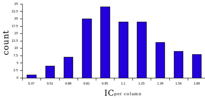
Figure 3: Jaspas motifs IC per column distribution.
