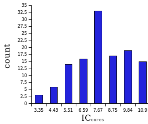
Figure 4: Jaspas cores IC distribution.
