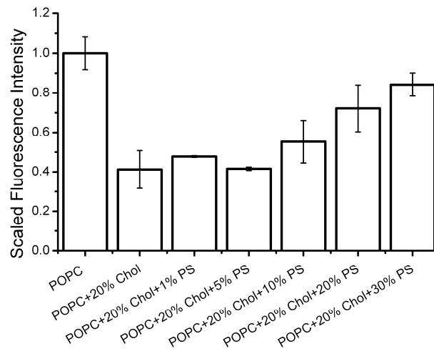
Figure S1. Scaled fluorescence intensities of Alexa647-labeled syntaxin-1A in lipid bilayers of different compositions. The fluorescence intensity in POPC:CHOL (4:1) is self-quenched as in Figure 1. Various additions of POPS relieve this self-quenching progressively as POPS is increased. All intensities are scaled to the syntaxin in POPC only fluorescence. The means and standard deviations from at least three independent reconstitutions for each condition are shown.
