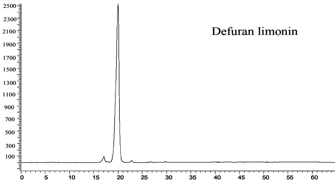
Figure 2S. HPLC chromatogram of modified compounds
