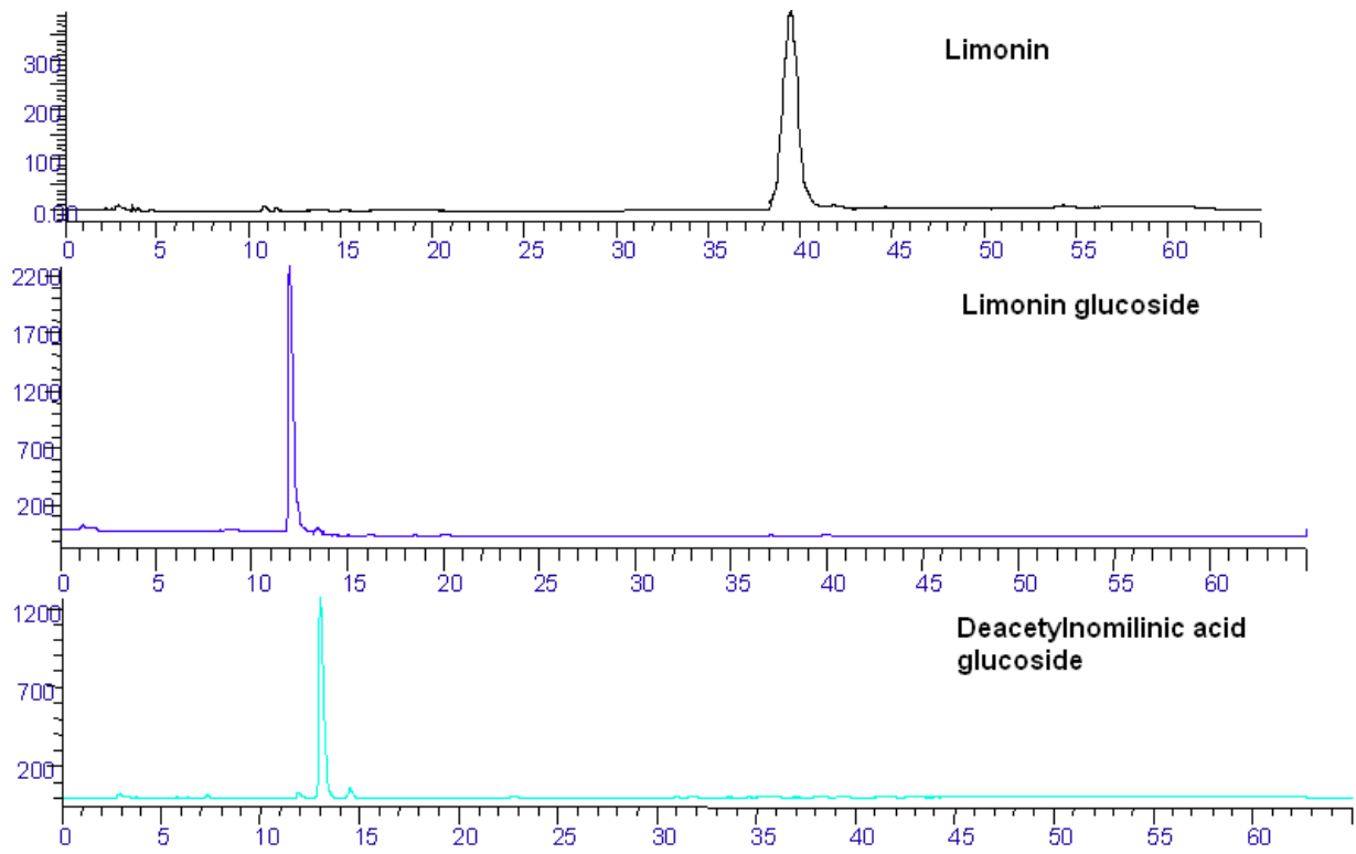
Figure 1S. HPLC chromatograms of purified citrus limonoids.
