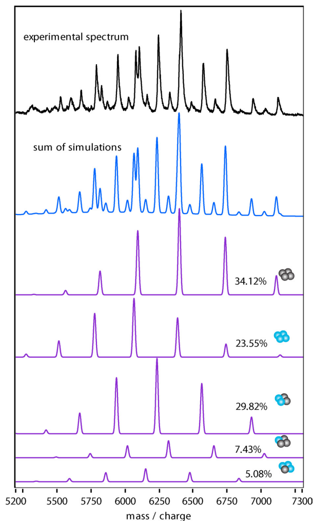
Fig. S1. Simulation of a selected mass spectrum (p53CT 37 °C after 5 h) the individual components are simulated separately (violet), so that the simulation (added component simulations plus simulated background, shown in blue) maximally resembles the measured mass spectrum (black).
