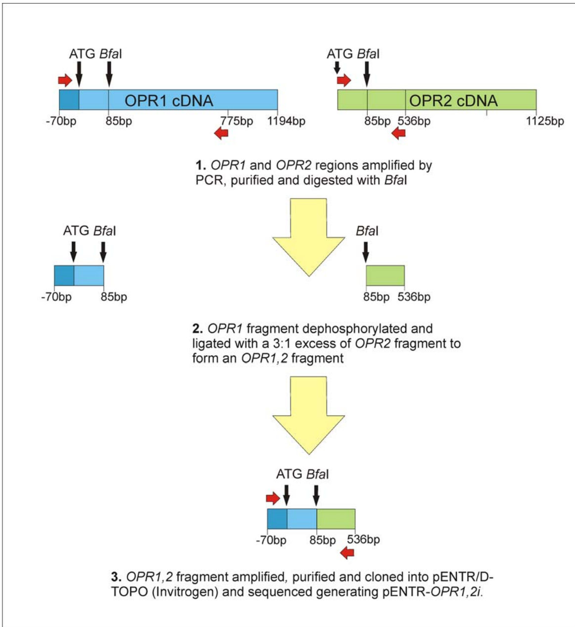
Figure S2 Construction of the RNAi OPR1,2i vector. The construct included a 155 bp region of OPR1 and 451 bp region of OPR2 , linked via a Bfal restriction site, to give a construct containing a 614 bp chimeric sequence of OPR1 and OPR2 .
