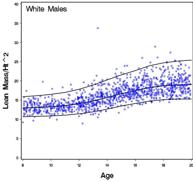
Figure S10: Lean Mass/Height 2 (kg/m 2 ) vs. Age in pediatrics. Solid lines indicate the 3 rd , 50 th , and 97 th percentiles.
