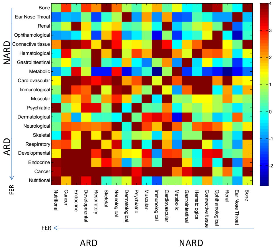
Figure S3: Z-score of closeness between different diseases. Here, we set values larger than four to be four to achieve better visualization.
