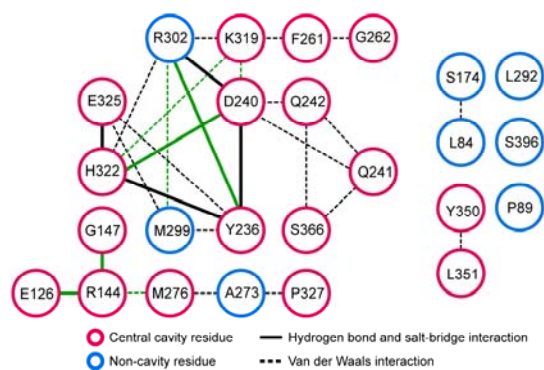
A. Ligand-free state (PDB ID: 2CFQ)
