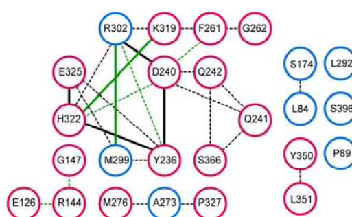
B. Ligand-bound state (PDB ID: 1PV7)
