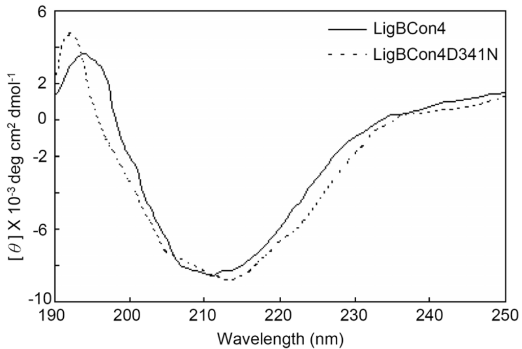
Supplemental Fig. 2 D341N mutation cannot affect the structure of LigBCon4
