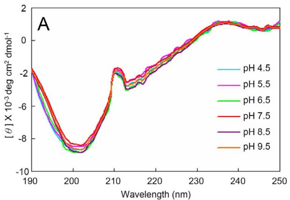
Supplemental Fig. 1 Environmental pH cannot affect the secondary structures of 17-27HTE and LigBCon4
