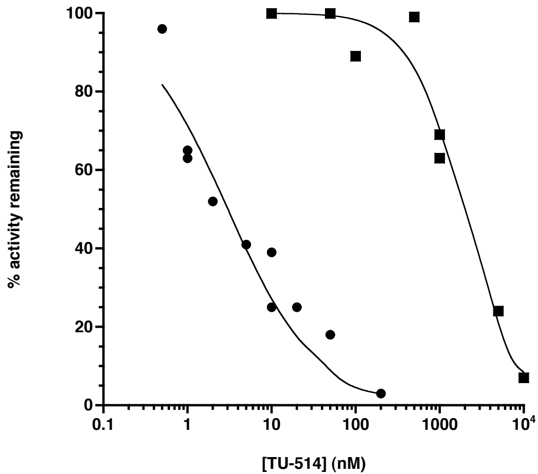
Supplemental Figure 1. Inhibition of AaLpxC by TU-514 at pH 7.4 or pH 5.5. The IC 50 of TU-514, determined at pH 7.4 (circles), is 2 nM, but at pH 5.5 (squares) it is 2 μM.
