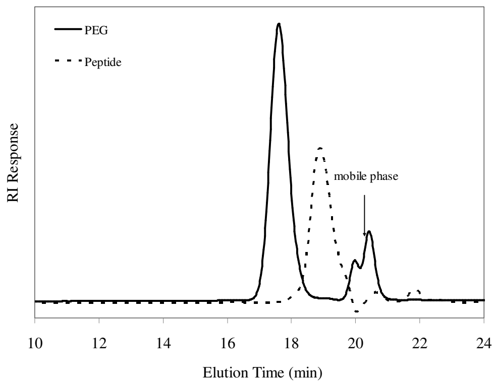
Figure S2. SEC analyses of PEG and peptide prepolymers. Mobile phase: PBS, pH=7.4, Refractive index detector.
