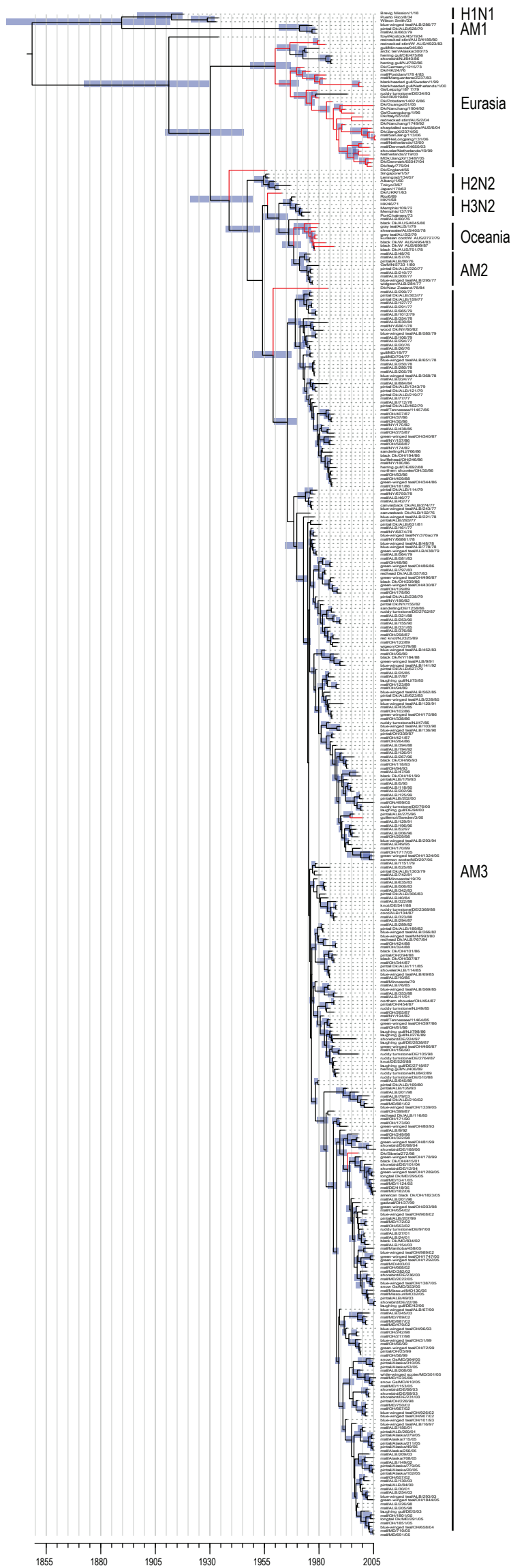
Figure S2. Dated phylogeny of the PB1 gene isolated from both Eurasia (red) and North America (black) Node bars indicate 95% HPD of divergence times. Scale bar shows timeline in years.
