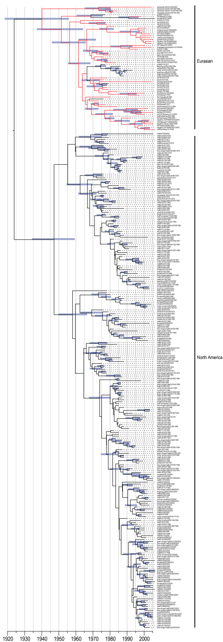
Figure S6. Dated phylogeny of the M gene isolated from both Eurasia (red) and North America (black) Node bars indicate 95% HPD of divergence times. Scale bar shows timeline in years.
