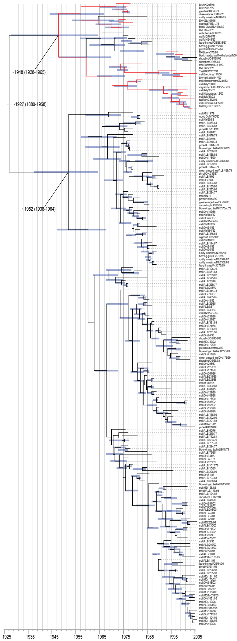
Figure S3. Dated phylogeny of the PB2 gene isolated from both Eurasia (red) and North America (black) Node bars indicate 95% HPD of divergence times. Scale bar shows timeline in years.
