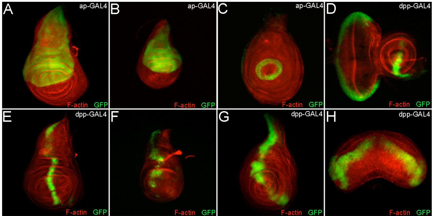
Supplemental Figure 1. Expression Pattern of ap-GAL4 and dpp-GAL4 drivers
