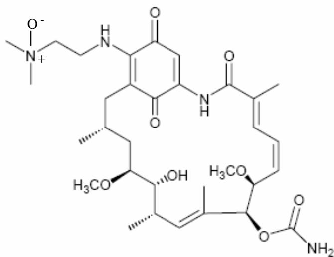
DMAG-N-oxide
