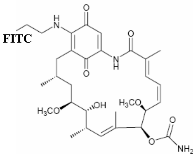
FITC-GA
