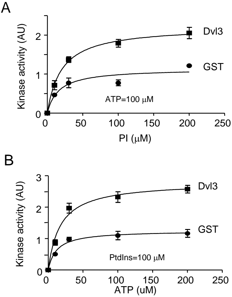
Figure S1. Representative kinase assays for Fig. 3B (A) and Fig. 3C (B). In these assays, 50 nM PI4KII \alpha was used with 100 nM Dvl or GST.
