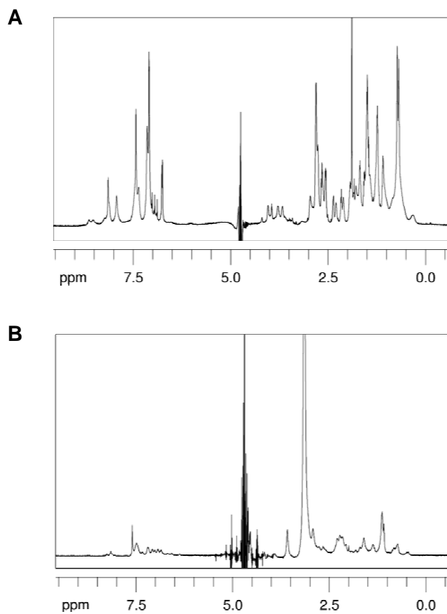
SUPPLEMENTARY FIGURE 1 D NMR spectra of warnericin RK. (A) 1.3 mM warnericin RK in sodium phosphate buffer, pH 5.6. (B) 1.4 mM warnericin RK in presence of 13.6 mM DMPC.
