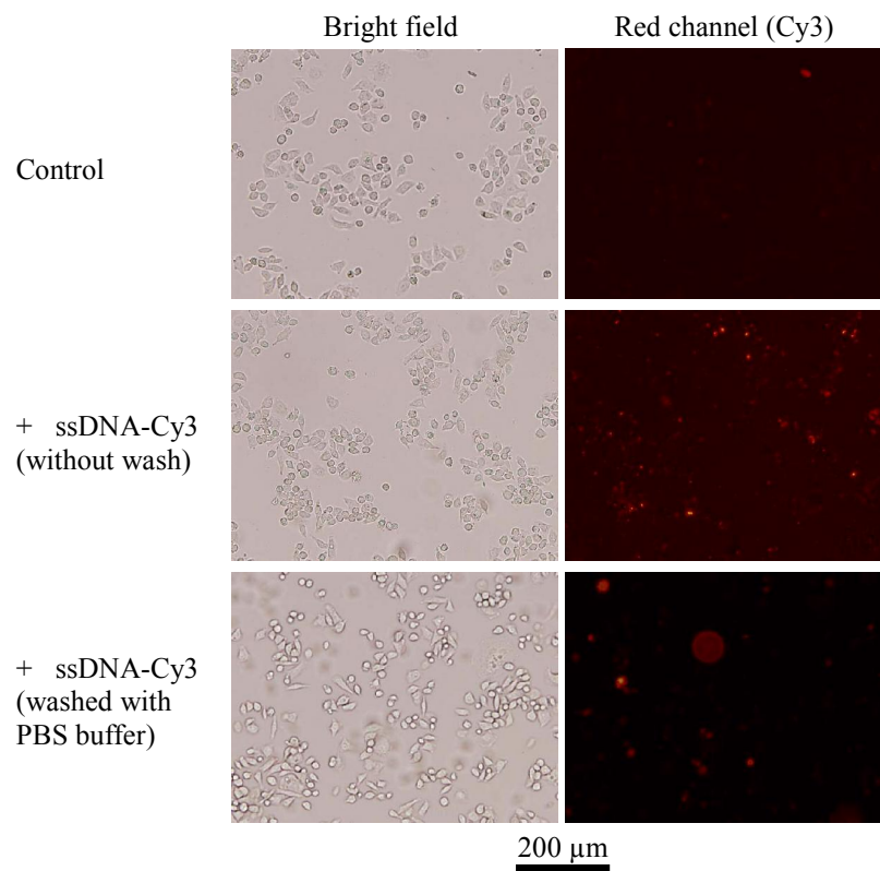
Figure S2. A control experiment shows that non-specific absorption of Cy3-DNA conjugates to cells can be easily washed off.
