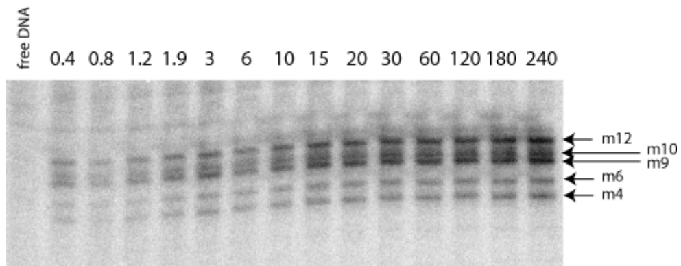
Supplementary Figure 6. Evolution of time-resolved potassium permanganate reactivity of the thymines on the template strand during formation of the RNAP-promoter complex. Representative gel of the reactivity pattern obtained upon mixing RNAP with consensus -10 T7A1 promoter for different amounts of mixing time, in seconds, shown above each lane.
