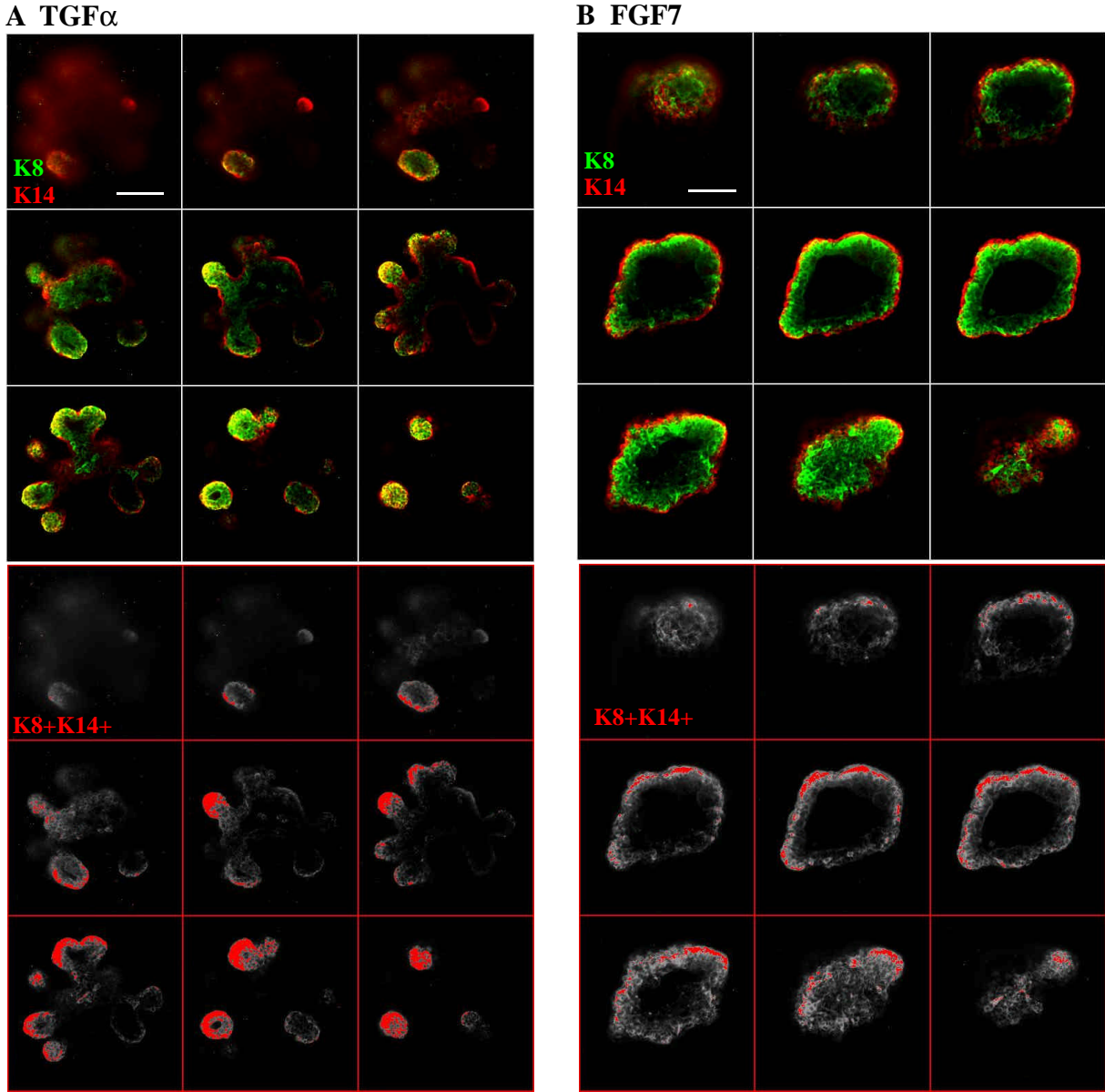
Supplemental Figure 1. Threshold analysis of K8+K14+ double positive cells.
