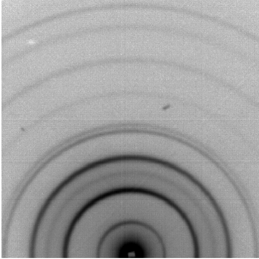
Figure 1S The ring-shaped diffraction pattern of a lipid mixture with PigCER:CHOL:FFA in a 2:1:1 molar ratio (see Table 1)
