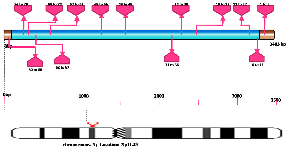
Fig SF51 - Schematic representation of miRNA target site hotspots on UBE1
