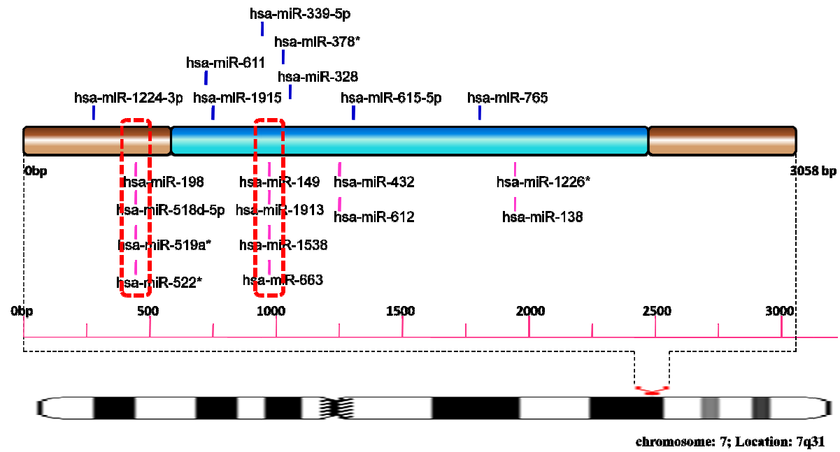
Fig SF5- Schematic representation of miRNA targets on GPR37
