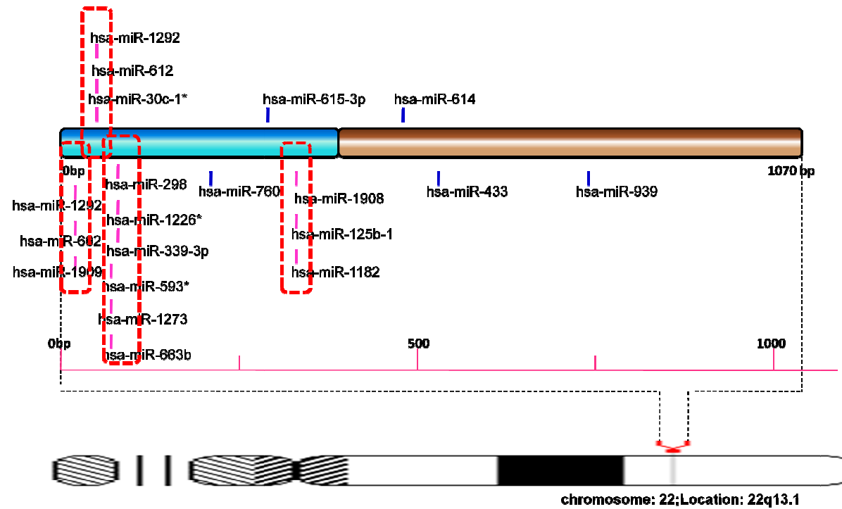
Fig SF8- Schematic representation of miRNA targets on LOC100128525
