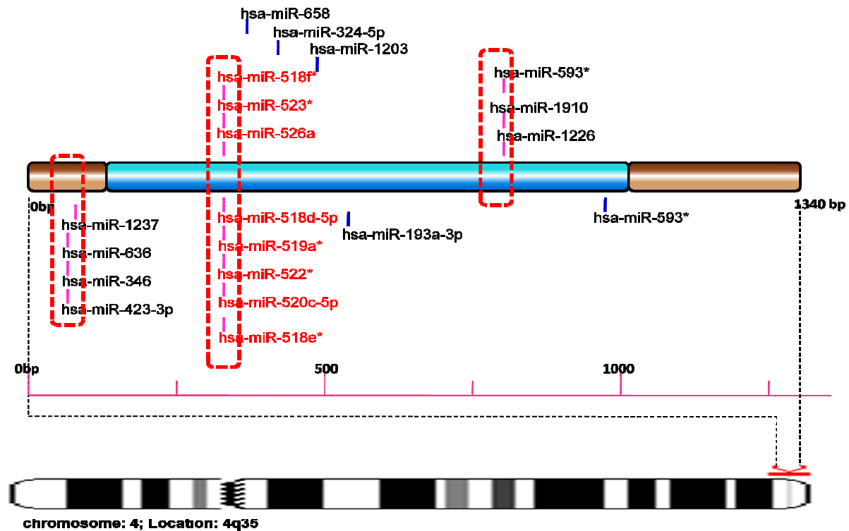
Fig SF19 - Schematic representation of miRNA targets on SLC25A4
