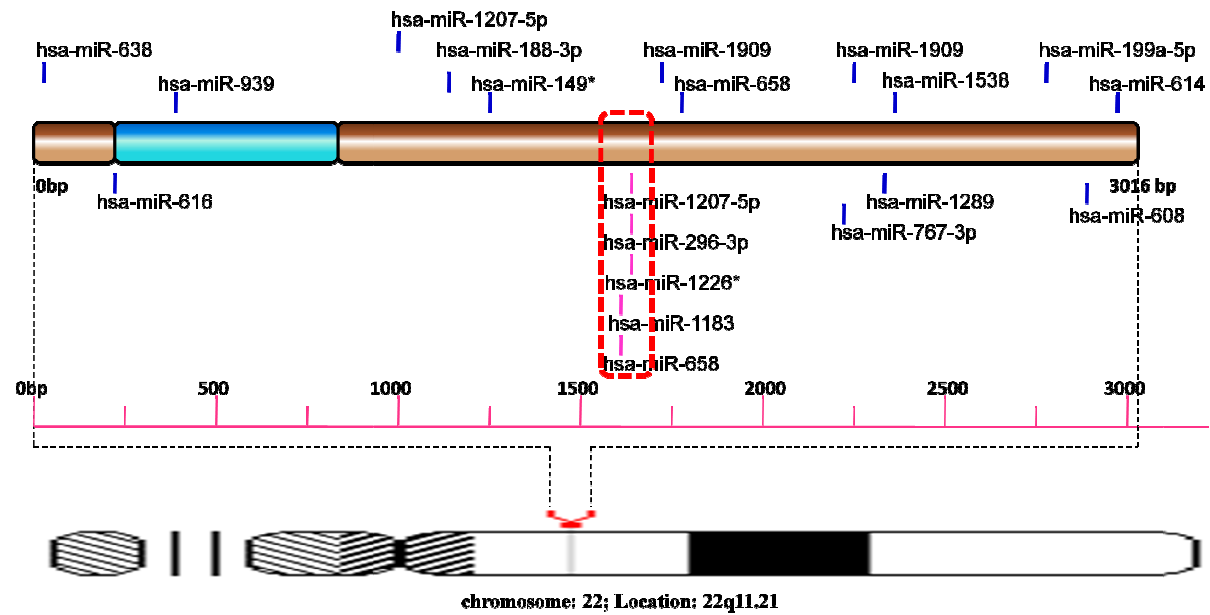
Fig SF25 - Schematic representation of miRNA targets on UBE2L3
