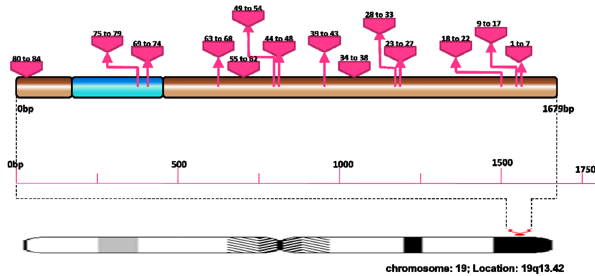
Fig SF32 - Schematic representation of miRNA target site hotspots on COX6B2
