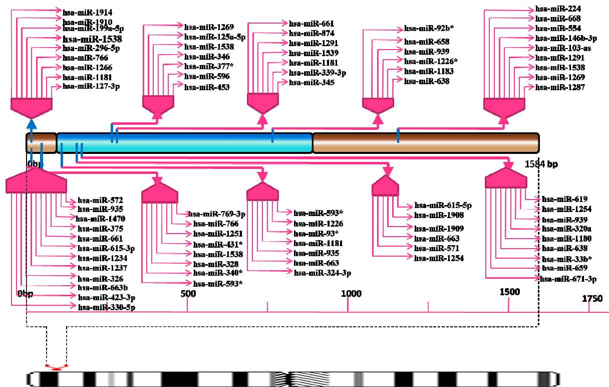
Fig SF31- Schematic representation of miRNA target site hotspots on ASP9
