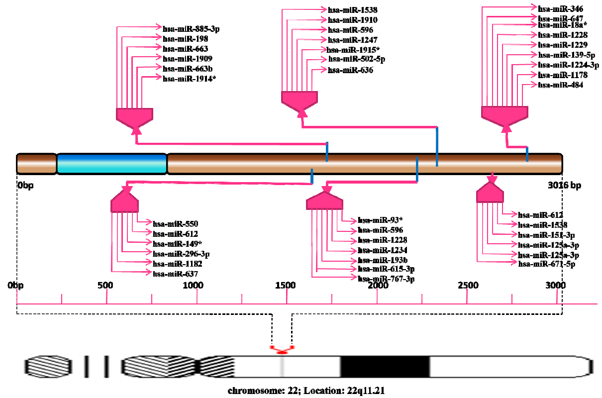
Fig SF53 - Schematic representation of miRNA target site hotspots on UBE2L3
