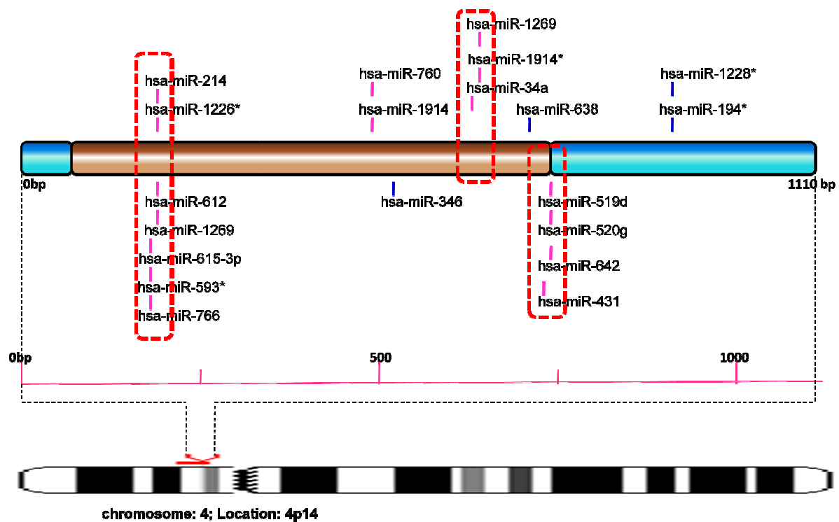
Fig SF27 - Schematic representation of miRNA targets on UCHL1
