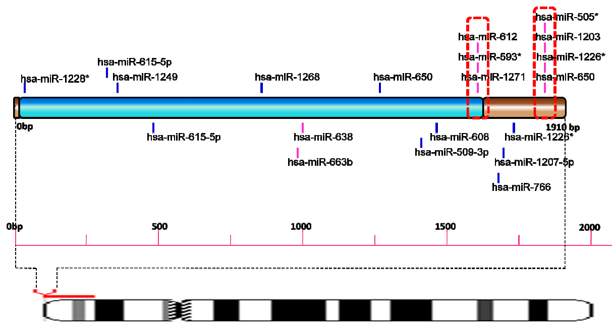
Fig SF22 - Schematic representation of miRNA targets on TH
