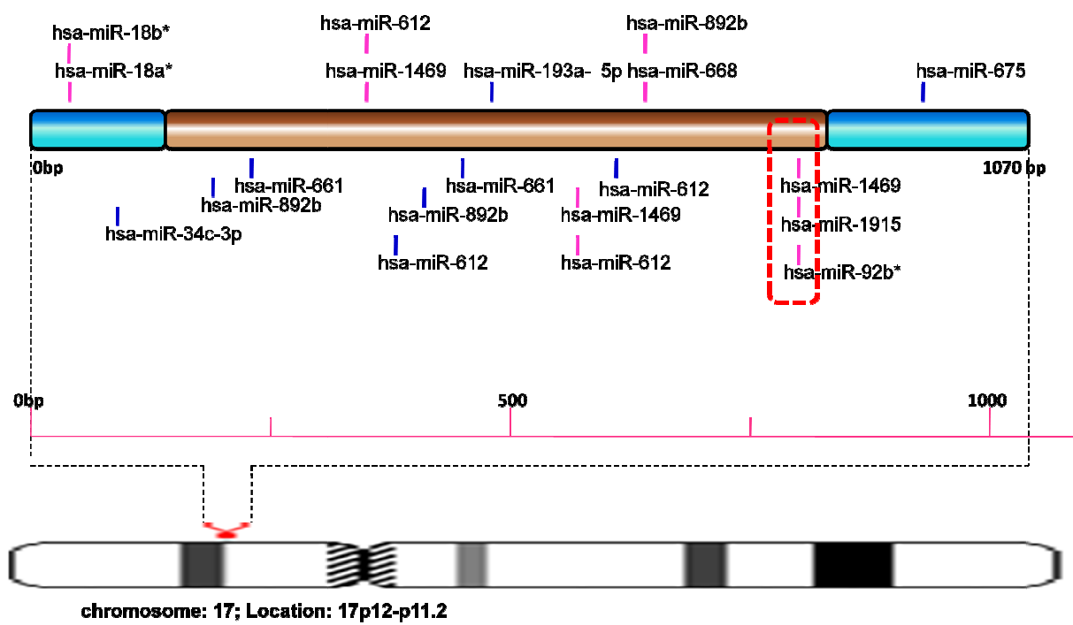
Fig SF26 - Schematic representation of miRNA targets on ubiquitinB
