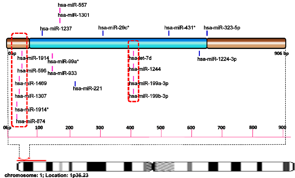
Fig SF13 - Schematic representation of miRNA targets on PARK7
