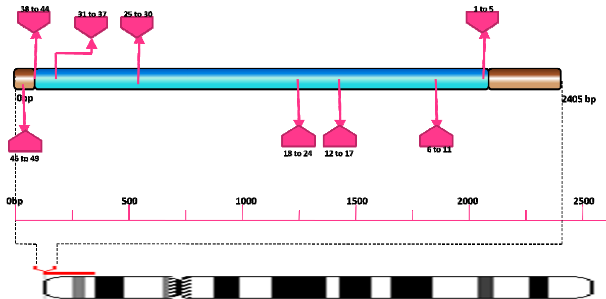
Fig SF 43- Schematic representation of miRNA target site hotspots on SDHA
