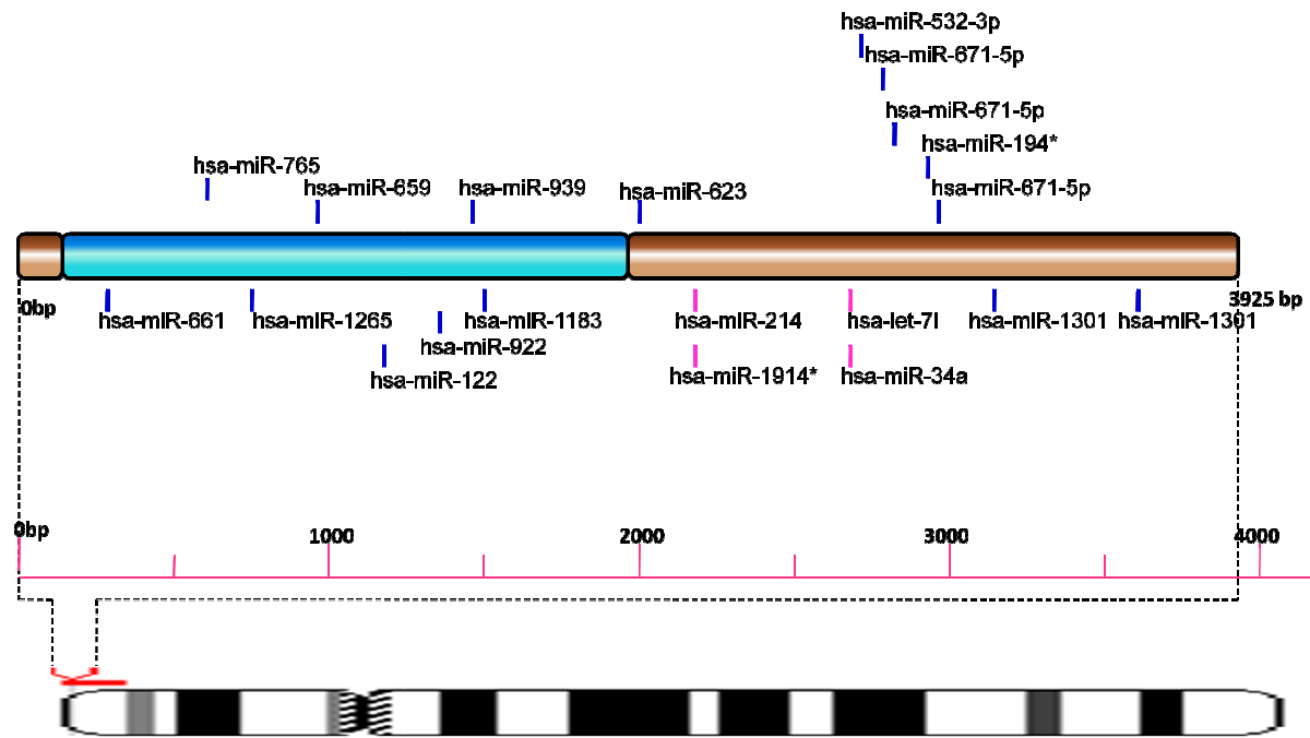
Fig SF17 - Schematic representation of miRNA targets on SLC6A3
