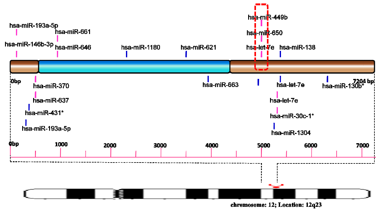
Fig SF7- Schematic representation of miRNA targets on APAF1
