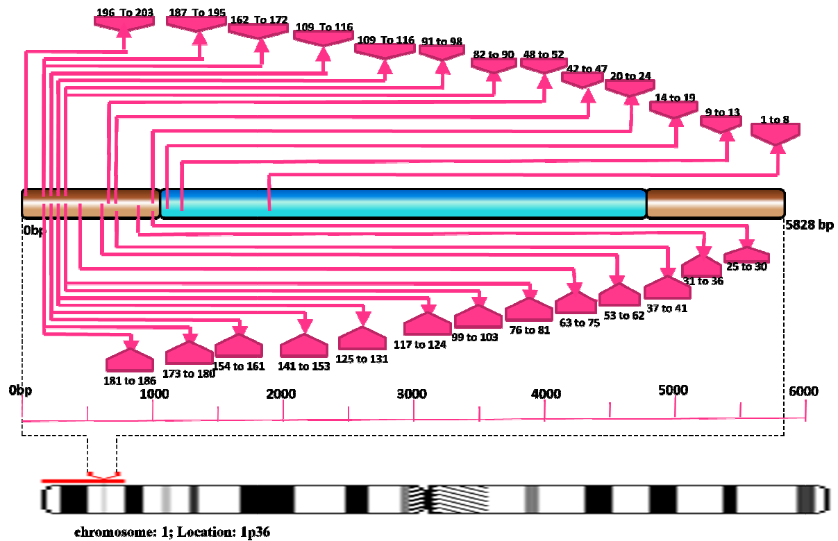
Fig SF 42 - Schematic representation of miRNA target site hotspots on PINK1
