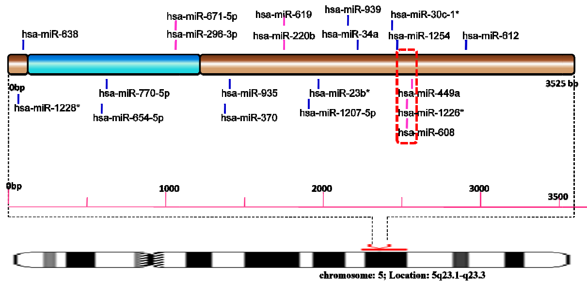
Fig SF21 - Schematic representation of miRNA targets on SNCAIP
