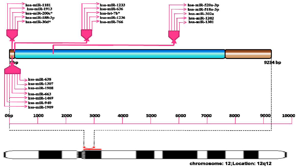
Fig SF38 - Schematic representation of miRNA target site hotspots on 10-LRRK2
