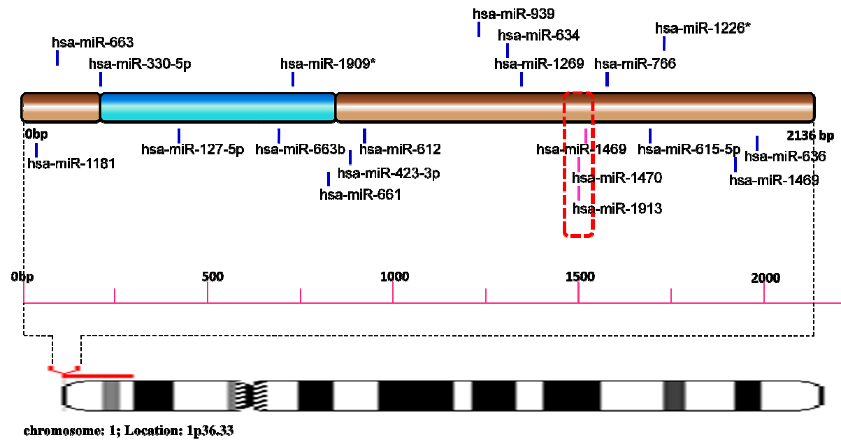
Fig SF24 - Schematic representation of miRNA targets on UBE2J2
