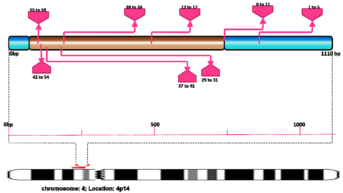
Fig SF55 - Schematic representation of miRNA target site hotspots on UCHL1
