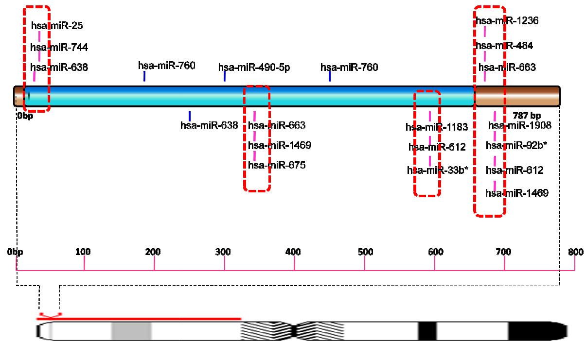
Fig SF11 - Schematic representation of miRNA targets on NDUFS7
