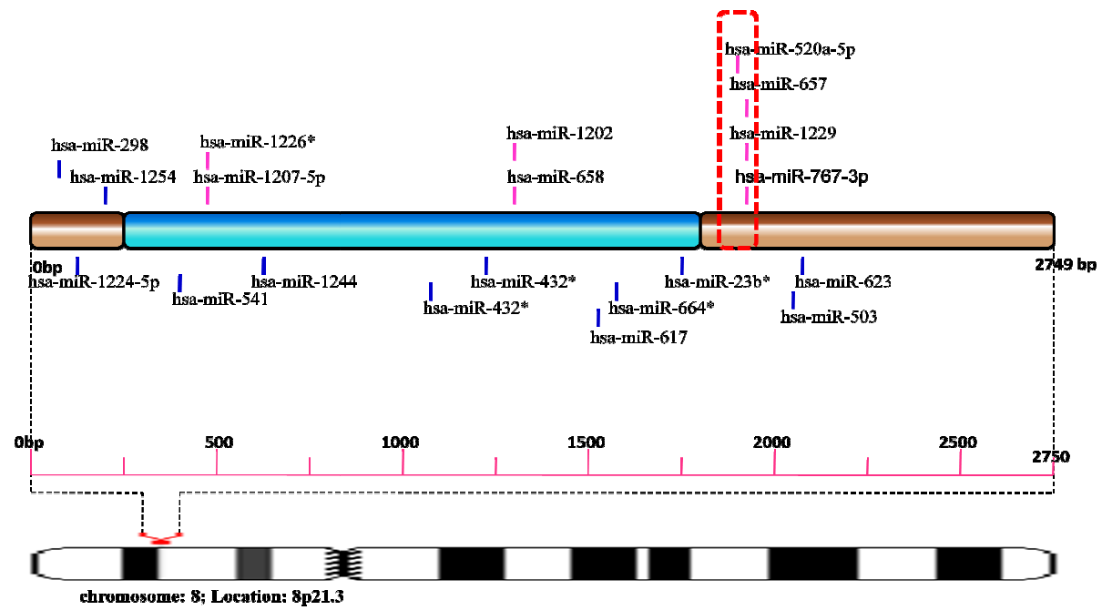
Fig SF18 - Schematic representation of miRNA targets on SLC18A1
