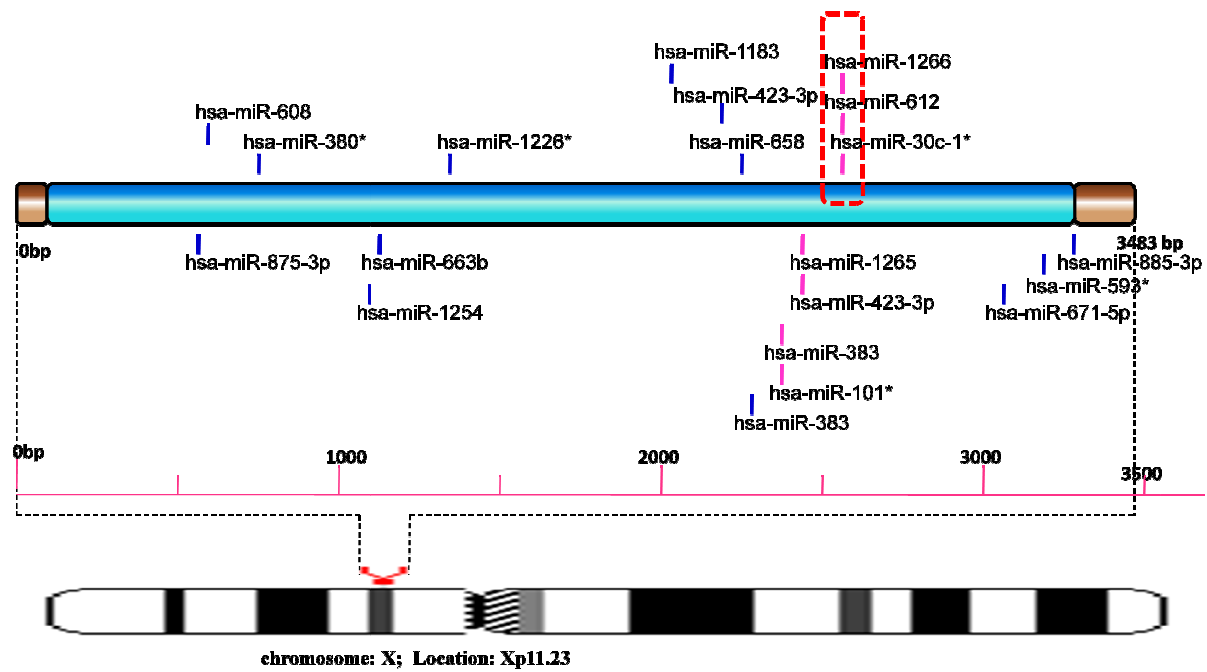
Fig SF23 - Schematic representation of miRNA targets on UBE1
