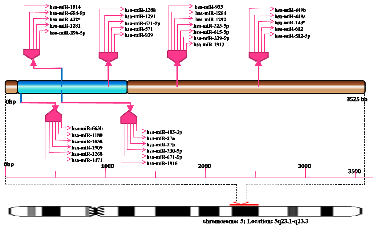
Fig SF49 - Schematic representation of miRNA target site hotspots on SNCAIP
