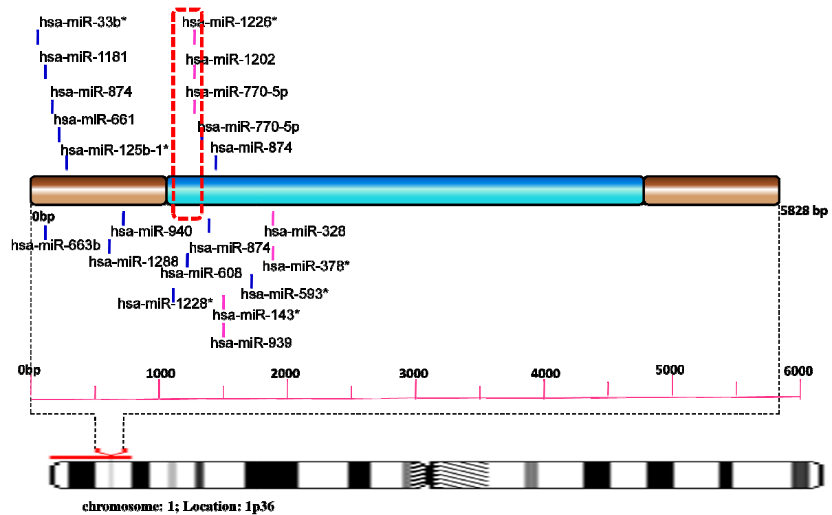
Fig SF14 - Schematic representation of miRNA targets on PINK1
