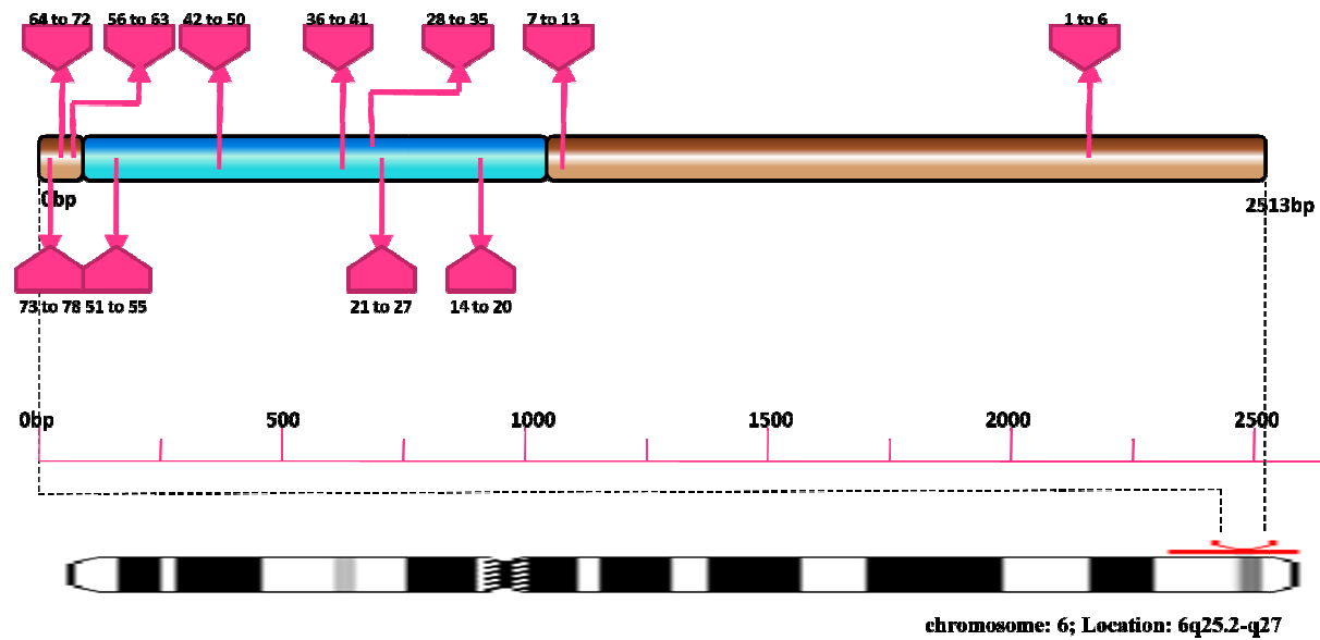
Fig SF40- Schematic representation of miRNA target site hotspots on PARK2
