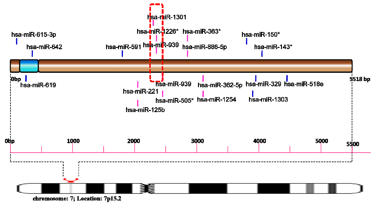
Fig SF4- Schematic representation of miRNA targets on CYCS
