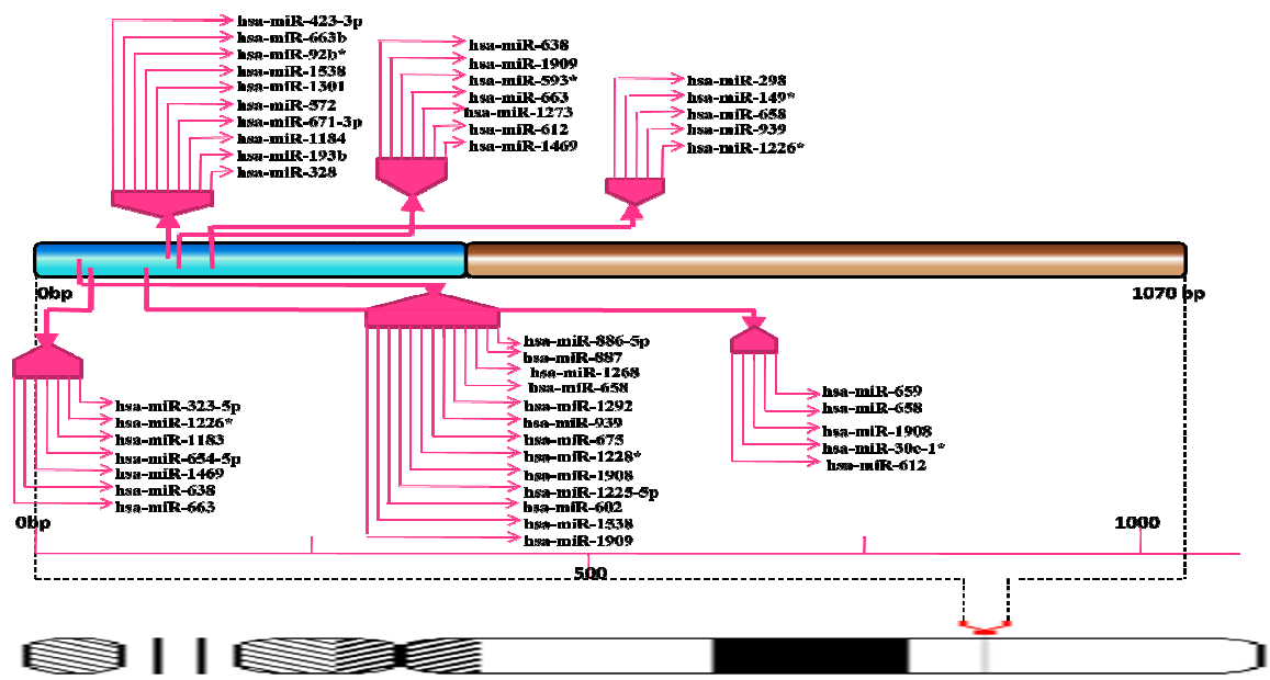
Fig SF37- Schematic representation of miRNA target site hotspots on LOC100128525
