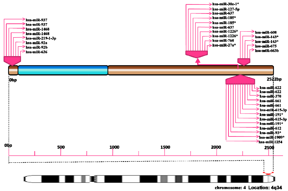
Fig SF30- Schematic representation of miRNA target site hotspots on CASP3
