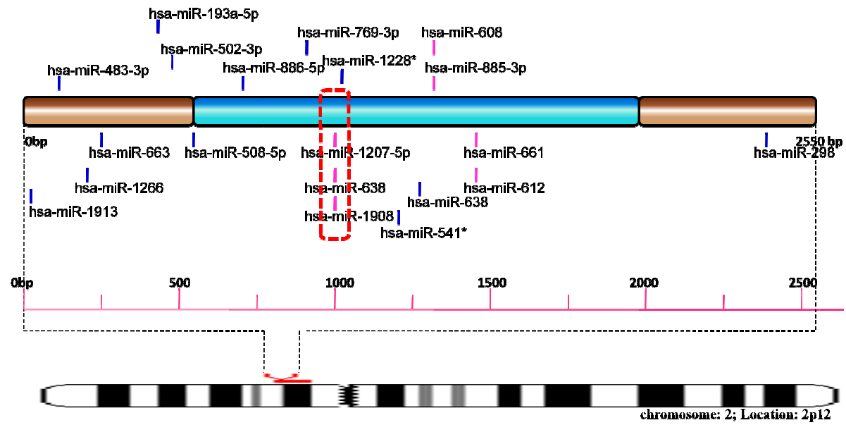
Fig SF6- Schematic representation of miRNA targets on HTRA2
