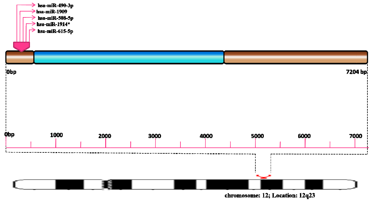
Fig SF36- Schematic representation of miRNA target site hotspots on APAF1
