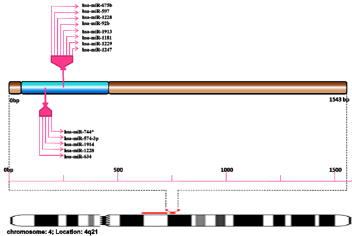
Fig SF48 - Schematic representation of miRNA target site hotspots on SNCA
