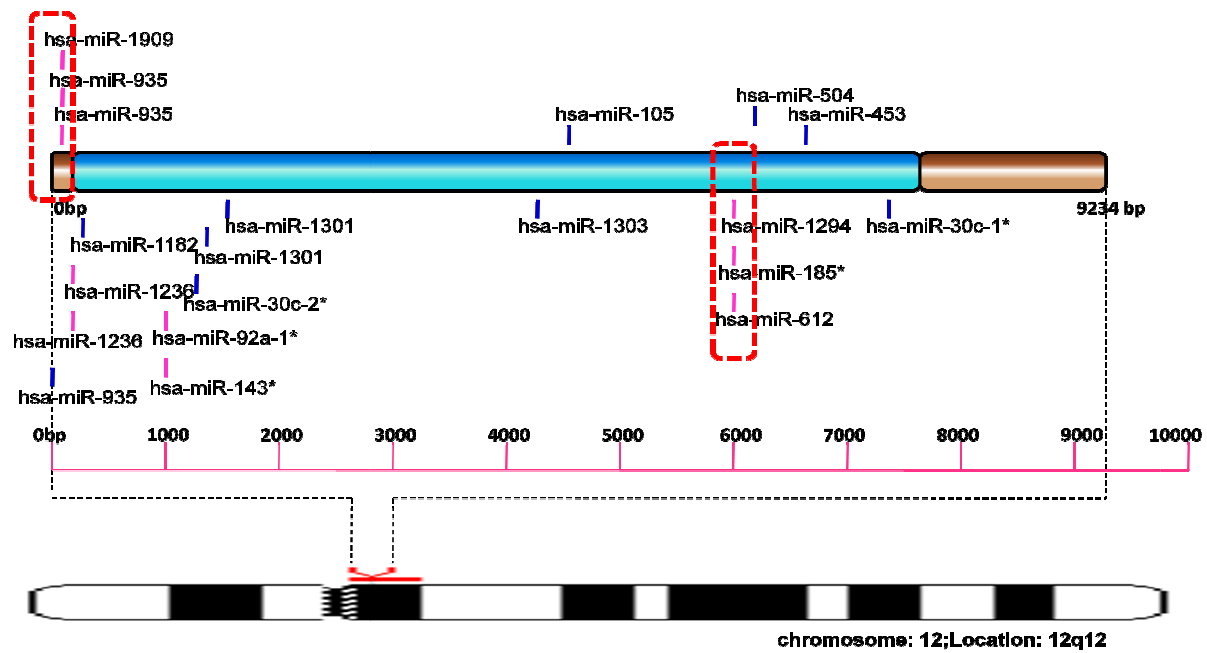
Fig SF10 - Schematic representation of miRNA targets on 10-LRRK2
