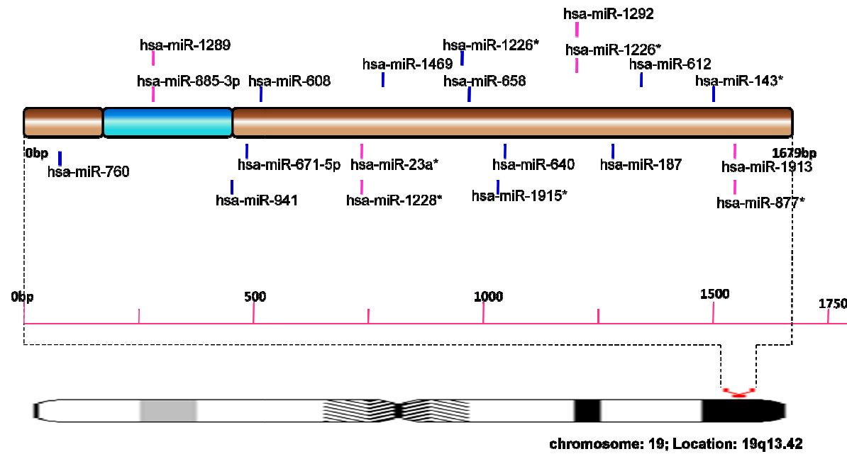
Fig SF3 - Schematic representation of miRNA targets on COX6B2
