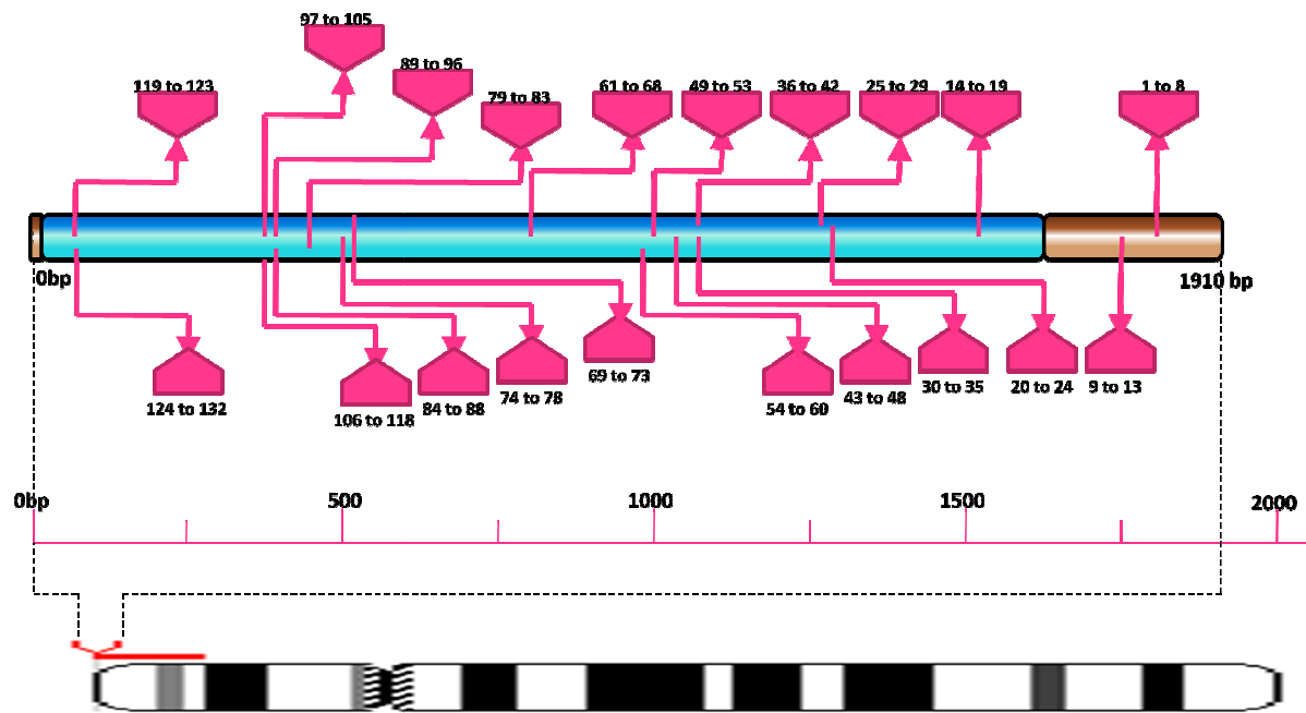
Fig SF50 - Schematic representation of miRNA target site hotspots on TH
