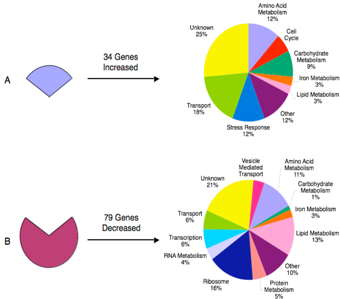
Supplementary Figure S2. Global expression changes in response to oleate. Schematic representing transcript levels in are1Δ are2Δ dga1Δ lro1Δ relative to control strains after a 6 hour exposure to 0.01mM oleate. Up-regulated (A) and down-regulated (B) genes are categorized by gene ontology.
