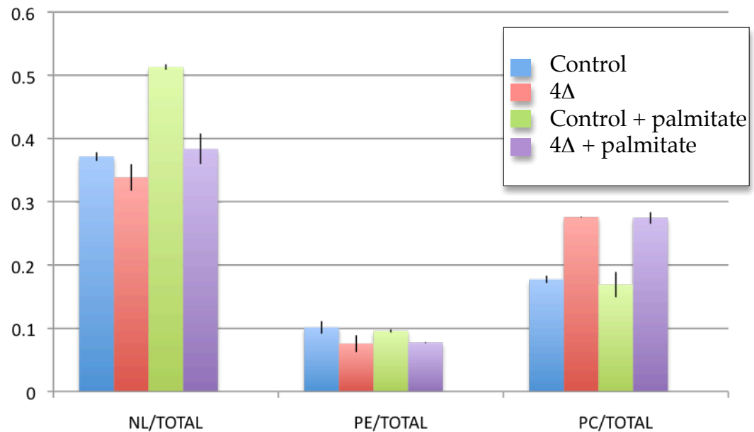
Supplementary Figure S3. Phospholipid composition of control (C) and Neutral lipid deficient (4Δ) strains. Lipids were extracted and resolved as described in experimental procedures and stained with Iodine. PE and PE represent phosphatidylethanolamine and phosphatidylcholine, respectively.
