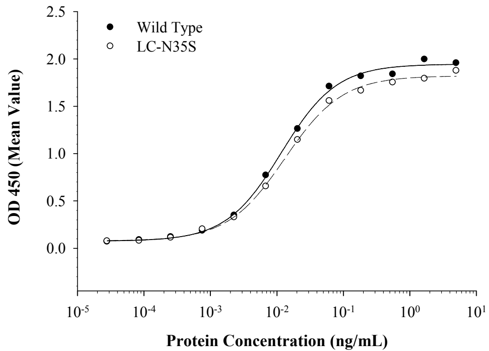
Supplemental Fig. 3. Binding of Antibody A to its antigen protein. Closed circles: the wild type (mAb A-1). Open circles: the protein with an Asn→Ser mutation at position 35 in the light chain.
