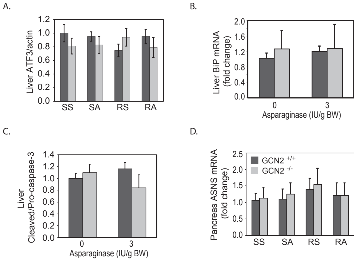
Figure S1. Neither asparaginase nor rapamycin altered hepatic expression of (A) ATF3, (B) BiP/Grp78 and (C) caspase-3 cleavage. (D) ASNS mRNA expression in pancreas was also not changed by either drug or genotype. Dark bars= wildtype GCN2 +/+ mice; light bars=GCN2 -/- null mice.
