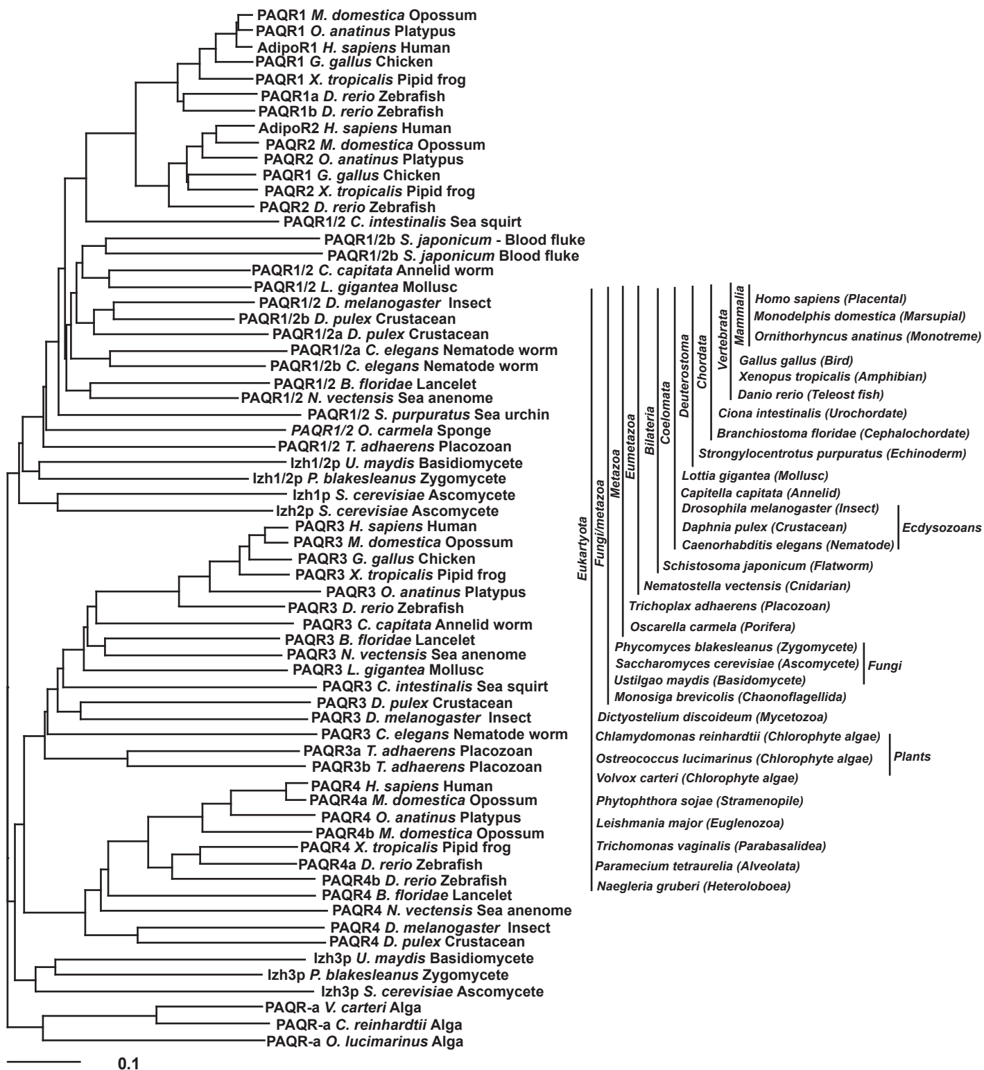
Supplemental Figure 1: Phylogenetic tree of Class I PAQRs. The tree is rooted with PAQR sequences from chlorophyte plants. On the right is a taxonomic key to the organisms from which these sequences and those in Figure 4 were derived.
