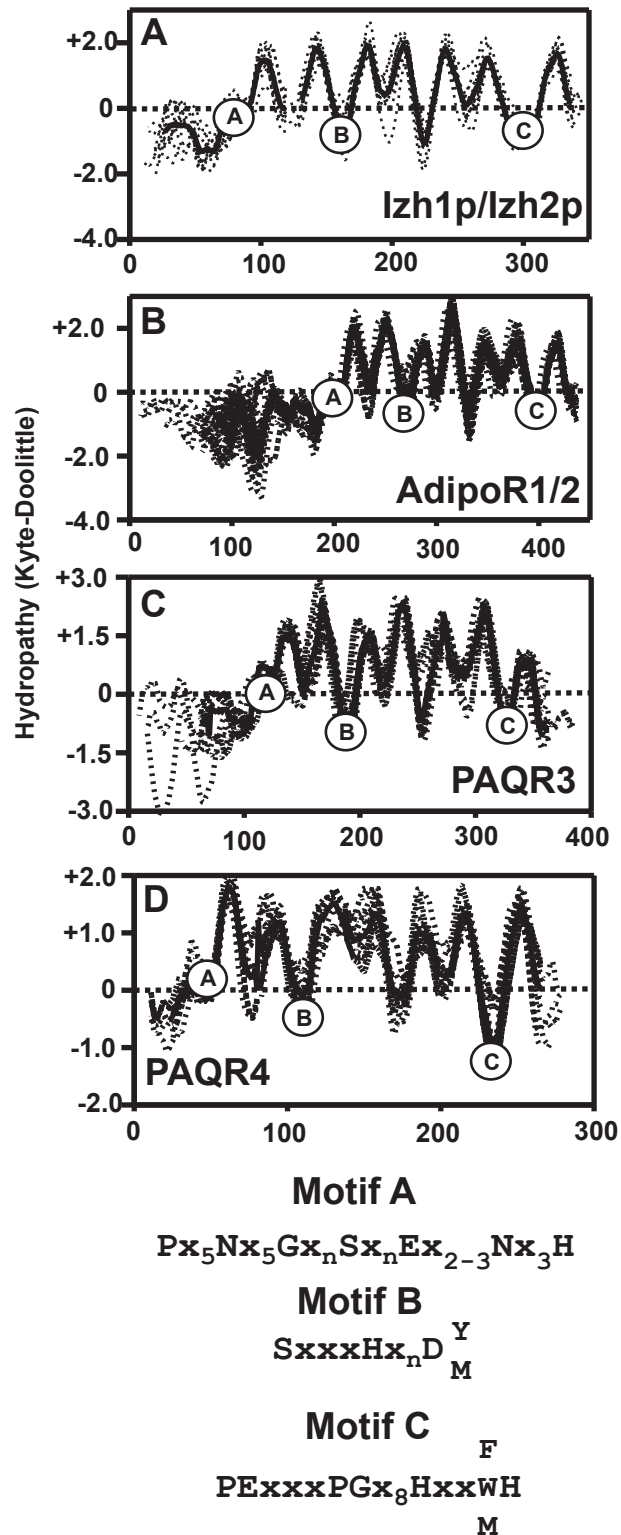
Supplemental Figure 3. Hydropathy plots for yeast and human Class I PAQRs. (A-D) Hydropathy plots for various individual proteins from different groups were generated and aligned (dotted lines). An average hydropathy plot for all members of each group were generated (solid lines). (A) Fungal Izh2p-like proteins. (B) Vertebrate AdipoR1/2-like proteins. (C) Vertebrate PAQR3-like proteins. (D) Vertebrate PAQR4-like proteins. (E) A topological model for all PAQRs with the positions of the three conserved motifs.
