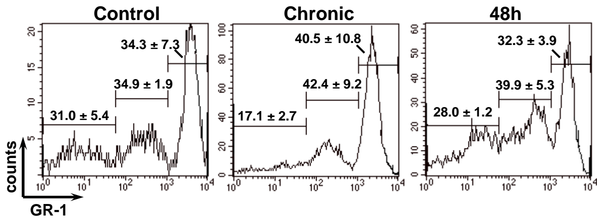
Supplementary figure S1 – GR-1 expression by Mac-1 + CD4 - CD8 - B220 - cells in the liver of unchallenged and challenged chronic mice. C57BL/6 mice infected for 7 months with T. cruzi parasites were challenged i.v. with 5x10 6 homologous trypomastigotes and, after 48 h, the liver leukocytes analyzed by flow cytometry. Control and chronic mice were also included. GR-1 expression by gated Mac1 + CD4 - CD8 - B220 - . Numbers indicate the mean ± SD of percentages of cells with low, intermediate and high GR-1 expression. Representative histograms of one experiment (n=3) out of two are shown.
