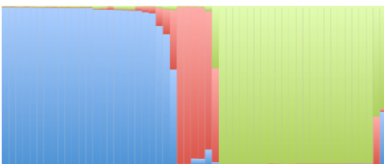
S pfs48/45 , K=3
