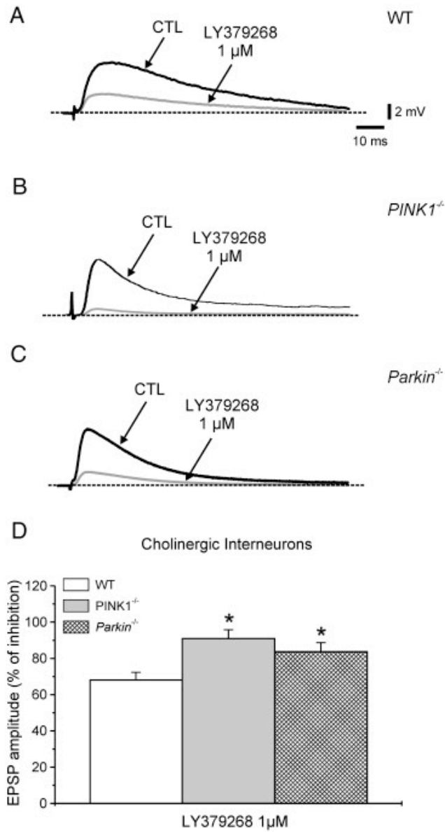
Fig. S1. Effect of LY379268 on striatal cholinergic interneurons. A. Sample traces of glutamate-mediated EPSPs recorded from a WT cholinergic interneurons. The superimposed trace shows the inhibitory effect of LY379268 (1 μM). The efficacy of LY379268 was significantly higher both in PINK1 -/- and Parkin -/- mice (B, C). D. The plot summarizes the inhibitory effects of LY379268 in the three strains of mice. Asterisk = p < 0.05 (one-way ANOVA, followed by post-hoc Tukey-test).
