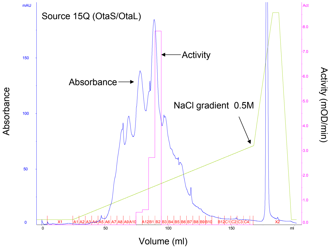
Supplemental Fig. 4. Chromatogram for the purification of OtaS/OtaL using a 10mL Source 15Q column
