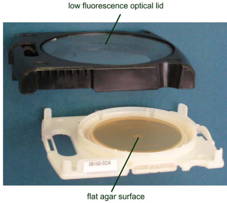
Figure S1. The growth cassette design enables efficient optical imaging of microcolonies.
