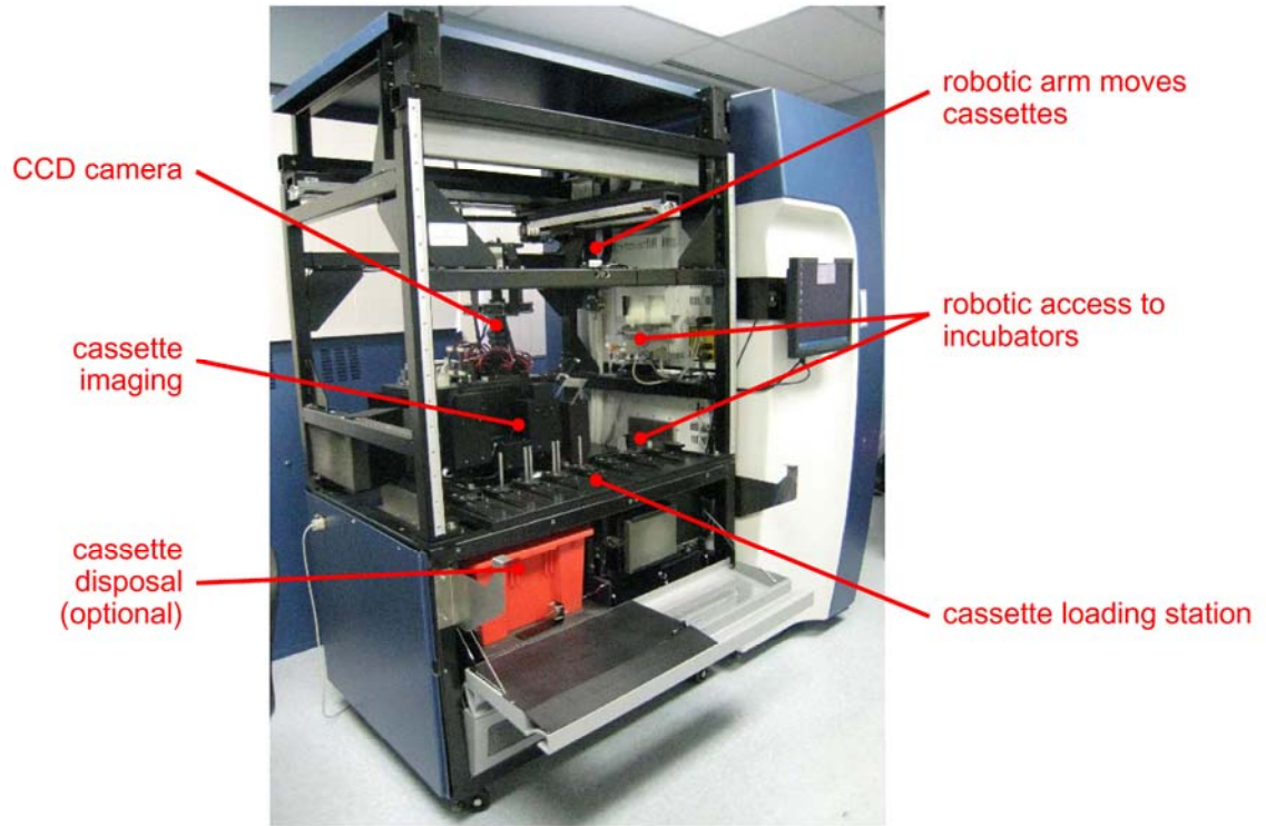
Figure S3. Key components of the Growth Direct System.
