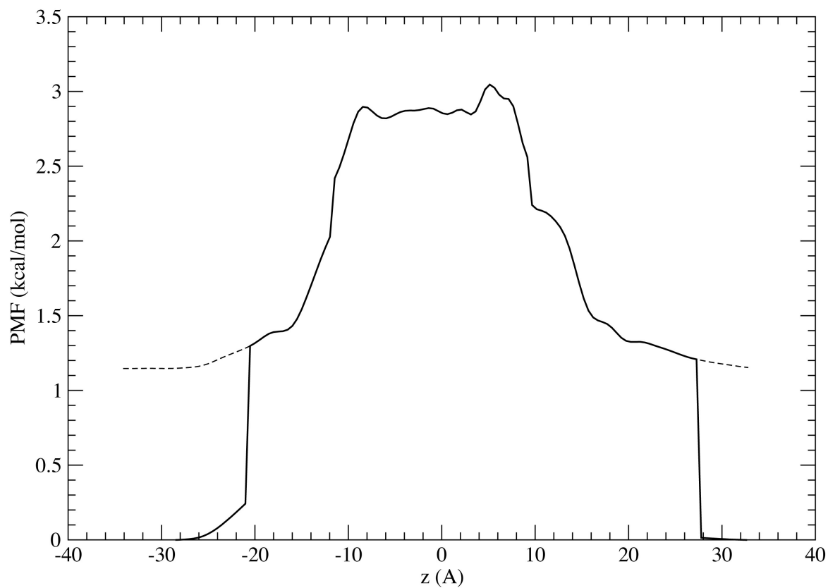
Figure S1: PMF of water permeation through AQP4 water pores. The PMF is obtained from averaged water occupancy in the four monomeric pores calculated using the 10-ns implicit ligand sampling simulation. The dashed line shows the PMF before correction for the entropy loss when water enters the channel.
