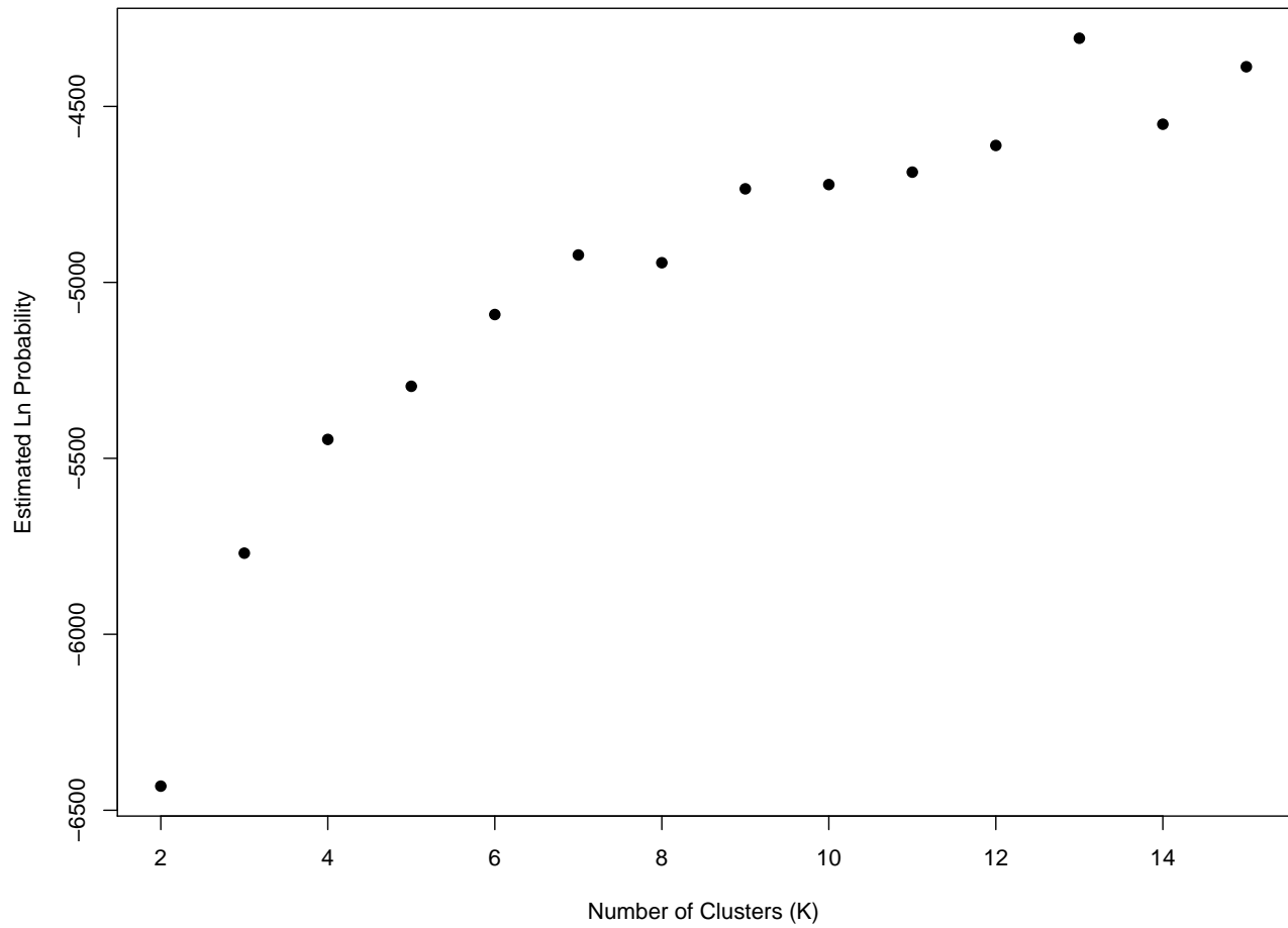
Figure S3: Probability of Different K Estimates: The estimated log probability of the data (as calculated by STRUCTURE) is plotted against different K values. For each K value, STRUCTURE was run 3 times, and the plotted value is the average of those 3 runs.
