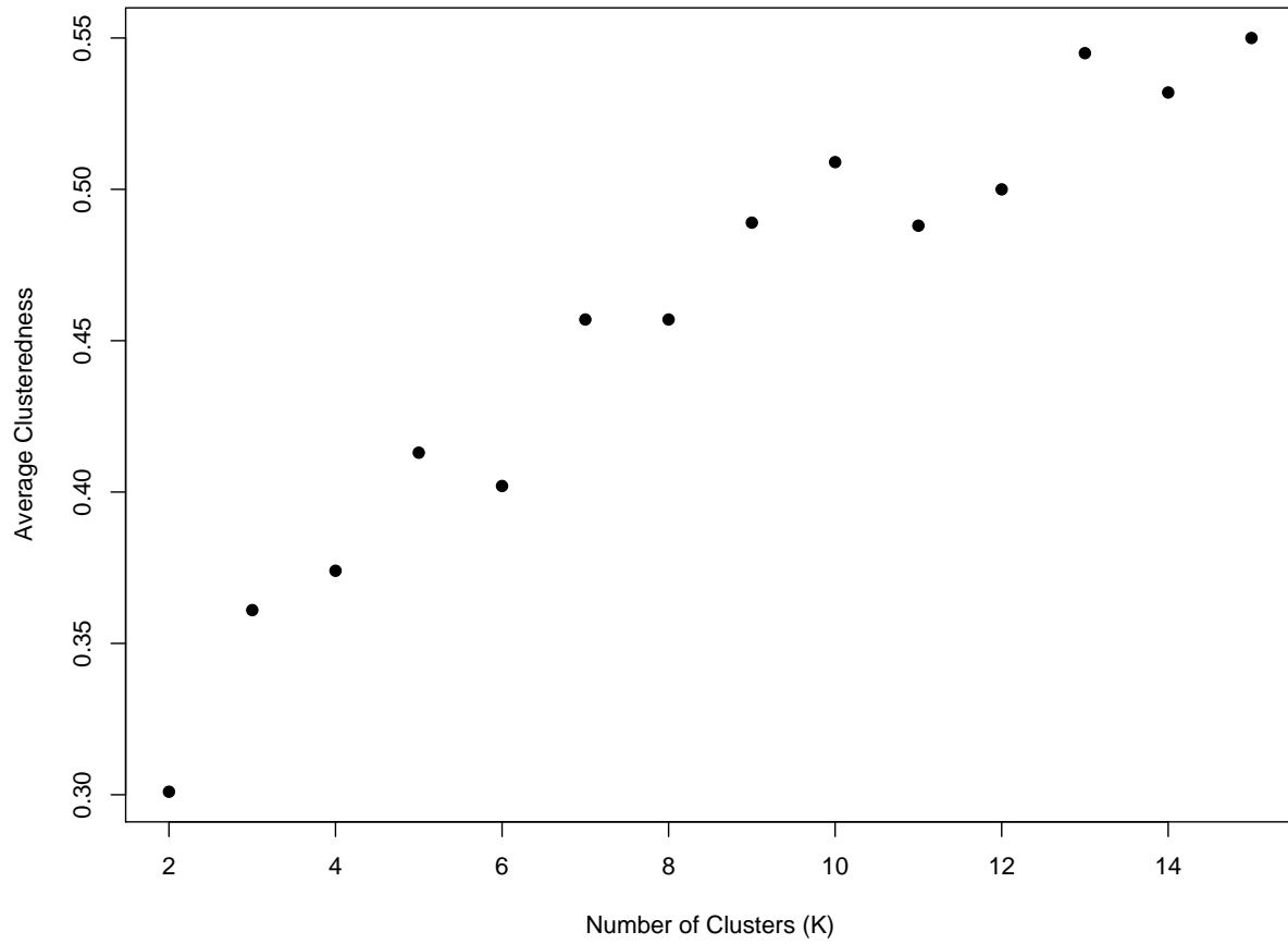
Figure S4: Average Clusteredness for Different K Values. For each K value, the average clusteredness measures the extent to which each individual belongs to a single cluster rather than to multiple clusters, so the higher the clusteredness the “better” the clusters.
