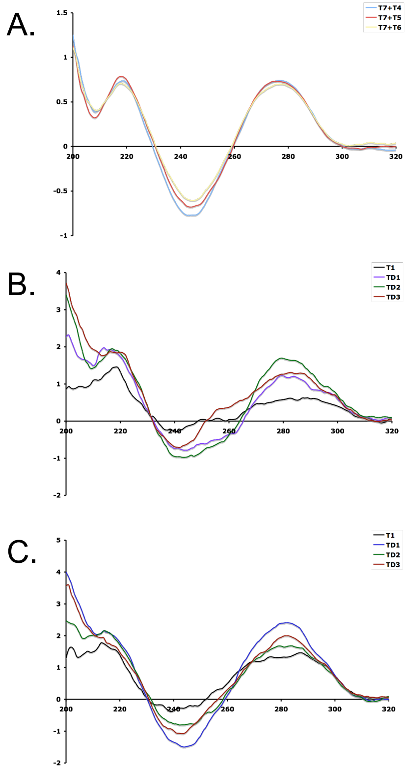
Supplemental Figure 1. Raw CD spectra of reference duplexes T7+T4 , T7+T5 and T7+T6 ( A ); telomeric oligonucleotide T1 and complexes TD1 , TD2 and TD3 measured in 100 mM Na + ( B ) or in 100 mM K + ( C ) solutions at 25 °C.
