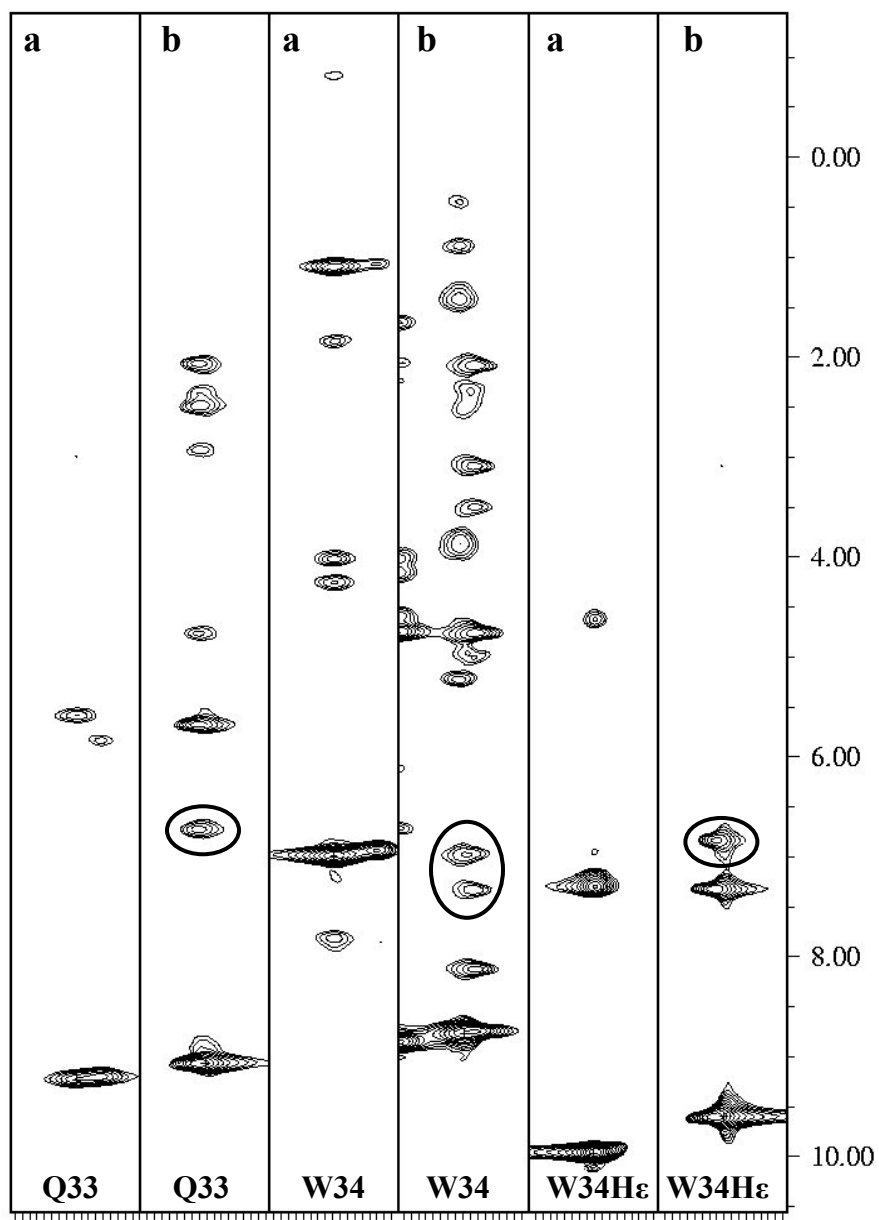
Supplementary Figure 1. Comparison of strips from 3D- N^{15} -NOESY spectra of Pin1 in absence (a) and in presence (b) of compound 29 (1:10 molar ratio Pin1/compound). Intermolecular NOE cross-peaks observed in the aromatic region (6.00 – 8.00 ppm) are circled.
