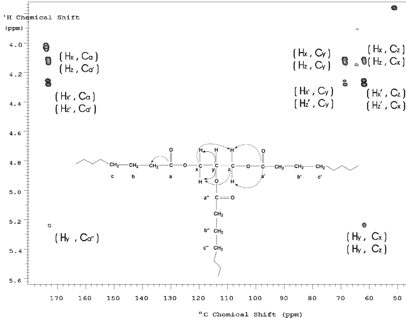
Figure A1. 2D HMBC contour plot of Compound 2, showing a long-range bonded network of ^1\text{H} - ^{13}\text{C} pairs and an isolated peak (4.03, 174 ppm) from an ester oligomer.
