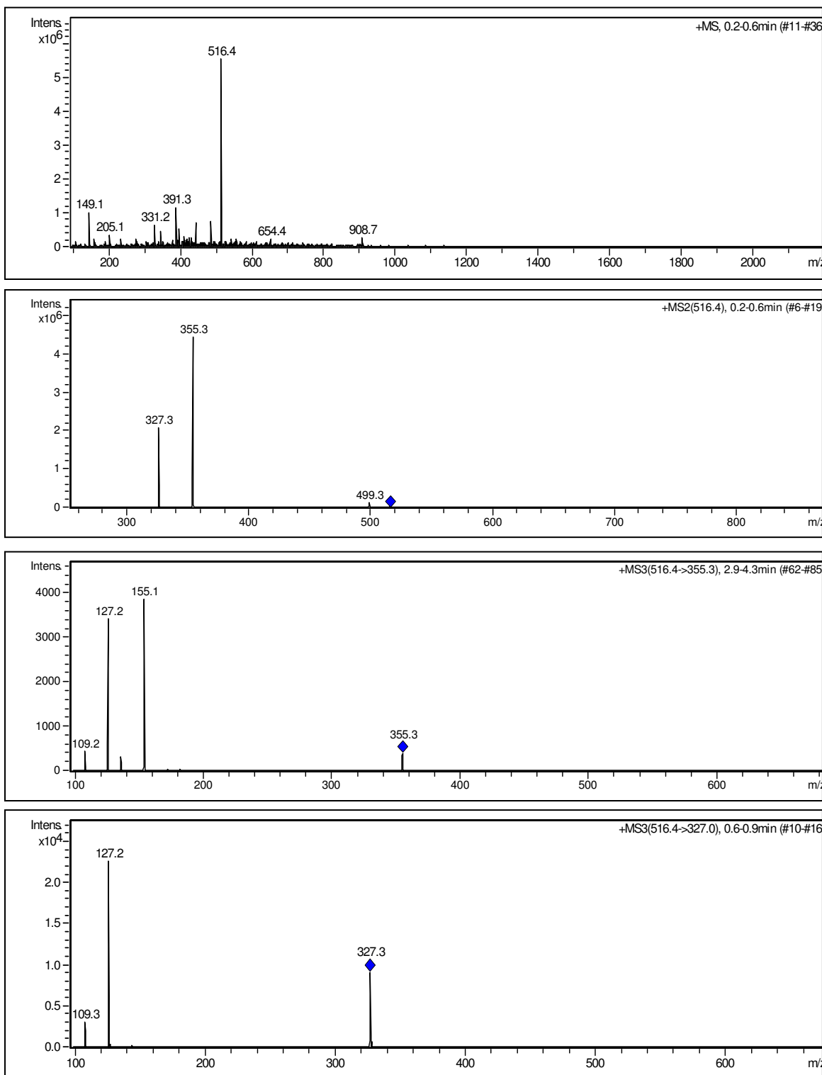
Figure A2. APCI-MS (top panel) and APCI-MS n (three bottom panels) of Compound 2 , plotted as ion intensity vs. mass-to-charge ratio.
