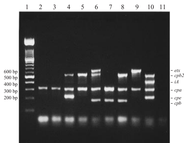
Fig. 1. Agarose gel electrophoresis of the PCR products obtained from the multiplex PCR assay for genotyping Clostridium perfringens and detection of the genes encoding enterotoxin and \beta 2-toxin. PCR products represent amplification of cpb (196 bp), cpe (233 bp), cpa (324 bp), iA (446 bp), cpb2 (567 bp) and etx (655 bp). Lanes: 1, DNA molecular weight markers; 2, C. perfringens NCTC 8237 (genotype A); 3, C. perfringens isolate 97-6 (genotype A); 4, C. perfringens PHLSARU 1289 (genotype Ae \beta 2); 5, C. perfringens NCTC 528 (genotype A \beta 2); 6, C. perfringens NCTC 4964 (genotype B \beta 2); 7, C. perfringens NCTC 3227 (genotype C); 8, C. perfringens NCTC 10719 (genotype C \beta 2); 9, C. perfringens NCTC 8503 (genotype D); 10, C. perfringens isolate 294 (genotype Ee \beta 2); 11, negative control (no template DNA).
