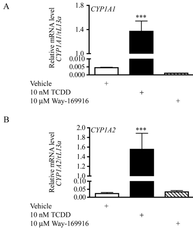
Supplemental figure 2. Way-169916 fails to induce AHR-dependent gene expression in MCF-7 cells.
