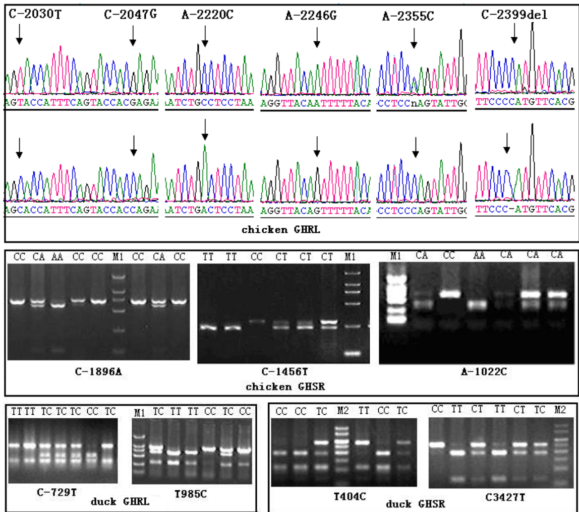
Supplemental Fig. 1. Genotyping profiles by sequencing and PCR-RFLP.
