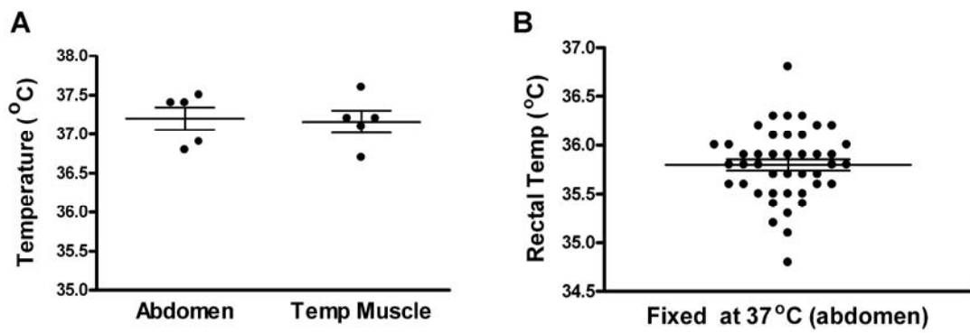
Figure 2S. Relationship among rectal, abdominal and brain temperature. A , Recordings of abdomen and temporal muscle in the head when a rectal temperature was fixed at 36.5°C as a set point. B , Recordings of rectal temperature when an abdomen temperature was fixed at 37°C as a set point.
