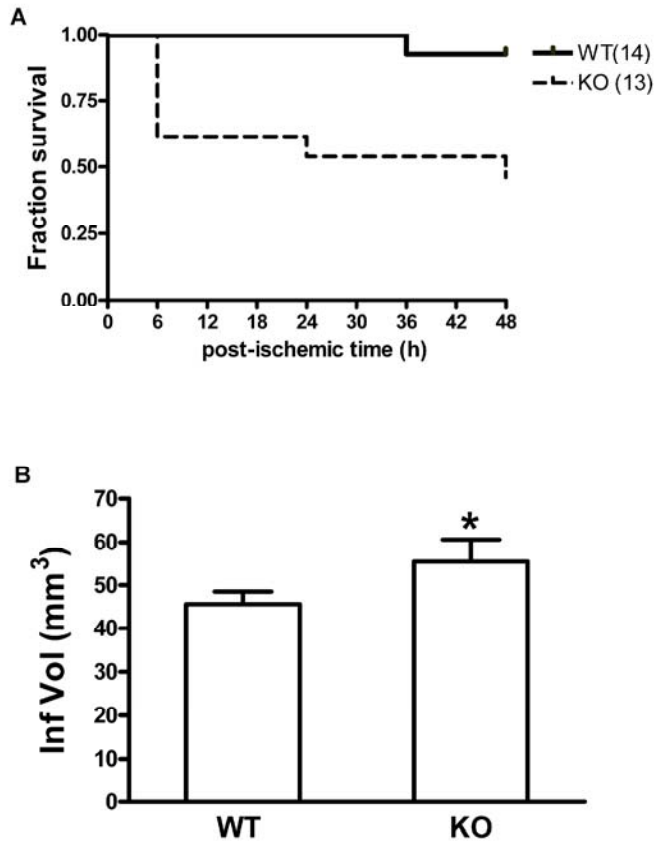
Figure 1S. High mortality (A) and enlarged infarct size (B) in hyperlipidemic mice. WT were fed ND and ApoE KO mice were fed HD for 8 weeks after wean. Infarct volume was measured 2 days after ischemia in survived mice (N=13 for WT, N=7 for KO). WT, wild type mice; KO, ApoE KO mice.
