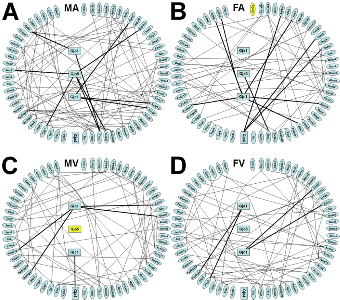
Supplementary Figure 1 Independently expressed HRD gene pairs in atria and ventricles of adult male and female mice. Note the sex and chamber differences in the significant expression decoupling of the selected genes. Yellow background for Gja5 in male ventricles and Scn5a in female atria indicates that these genes were excluded from the analysis in the indicated samples.
