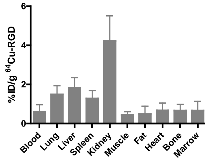
Supplementary Figure 1. Radiopharmaceutical retention in Tax + mouse tissues at 1 h p.i. Uptake in the kidney is high suggesting renal clearance as the main route of excretion.
