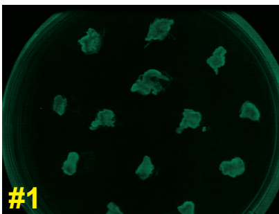
35S core
