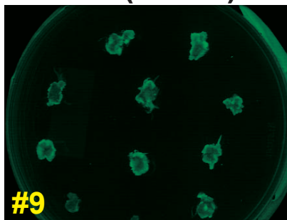
Untransformed
