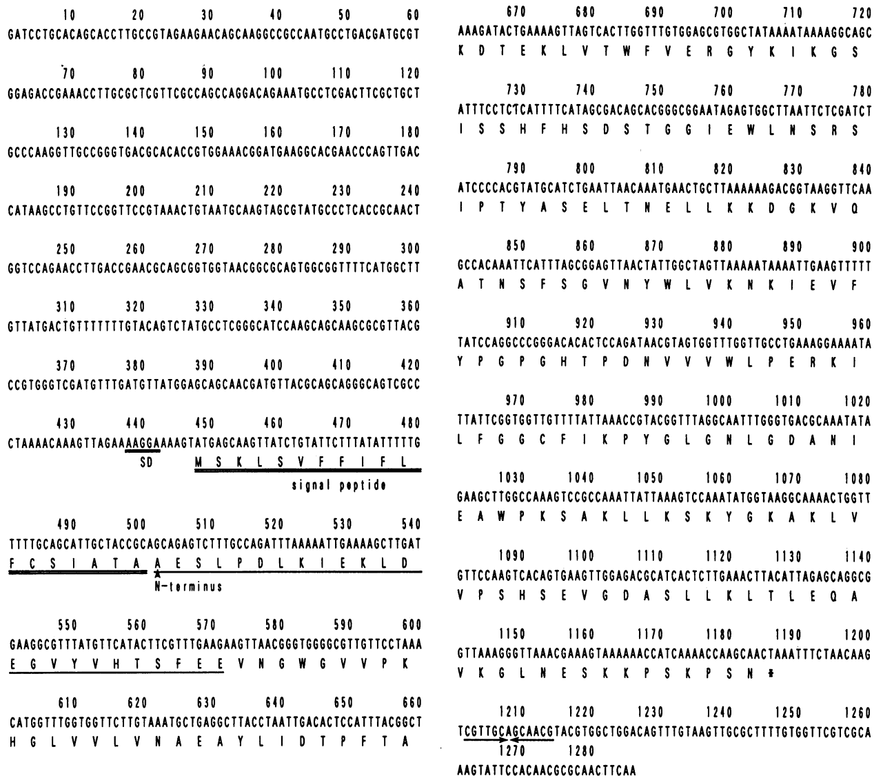
FIG. 2. Nucleotide sequence of bla IMP and its flanking regions. The deduced amino acid sequence is shown in the usual single-letter amino acid code below the nucleotide sequence. The putative Shine-Dalgarno sequence (SD) for bla IMP is underlined with a thick line, a 24-amino-acid sequence determined at the N terminus of a purified IMP-1 preparation is underlined, and the signal sequence of IMP-1 is double underlined. The N terminus of mature IMP-1 is marked with an arrowhead. Horizontal arrows indicate regions of dyad symmetry.
