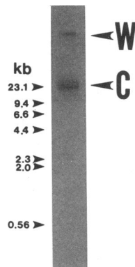
FIG. 5. Results from Southern hybridization. The 0.5-kb Hind III fragment of pSMBNU24 was used as a DNA probe. Chromosomal DNA was prepared from S. marcescens TN9106. C and W indicate the positions of chromosomal DNA and well, respectively, on the agarose gel.
