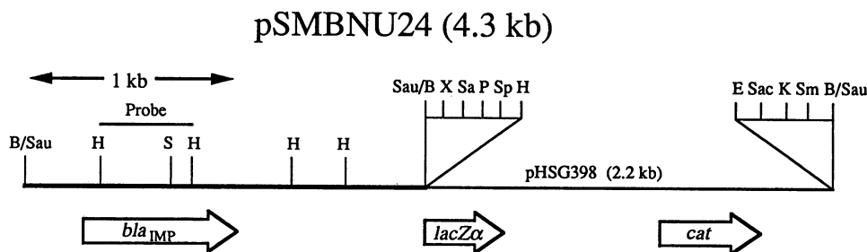
FIG. 1. Restriction map of pSMBNU24. The position and transcriptional direction of bla IMP are shown by an open arrow, as are those of the chloramphenicol acetyltransferase gene ( cat ) and 3'-truncated lacZ gene ( lacZ \alpha ) on the vector plasmid pHSG398 (31), which is shown by a thick line. Abbreviations: B, Bam HI; E, Eco RI; H, Hind III; K, Kpn I; Sa, Sal I; Sac, Sac I; Sau, Sau 3AI; Sm, Sma I; Sp, Sph I; P, Pst I; X, Xba I.
