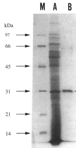
FIG. 4. Results from SDS-PAGE of purified IMP-1. Lanes: A, crude enzyme; B, purified IMP-1; M, molecular weight marker. The position of IMP-1 is indicated by an arrowhead.
