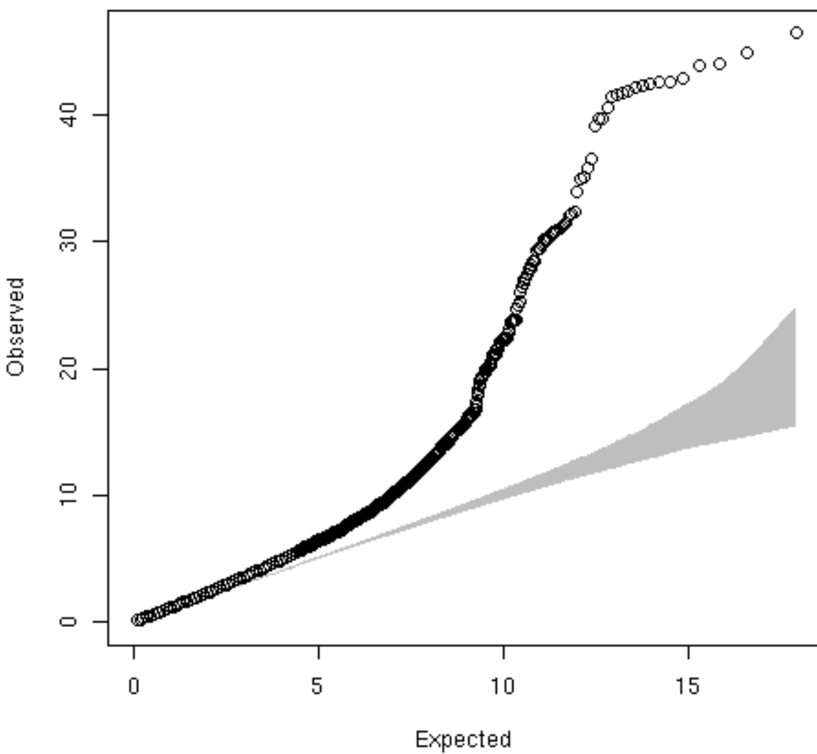
Stratified UK+Aus, lambda=1.14
